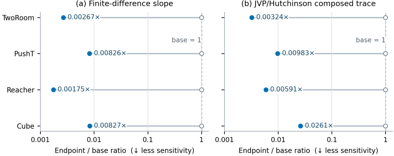
Figure 7: Local-sensitivity ratio of the checkpoint trained with Gaussian augmentation to the unaugmented checkpoint, estimated by finite differences and by a JVP/Hutchinson estimate of the composed Jacobian trace. Values below one indicate contraction after augmentation. The two estimators agree in direction for every task; these ratios do not establish task performance.
