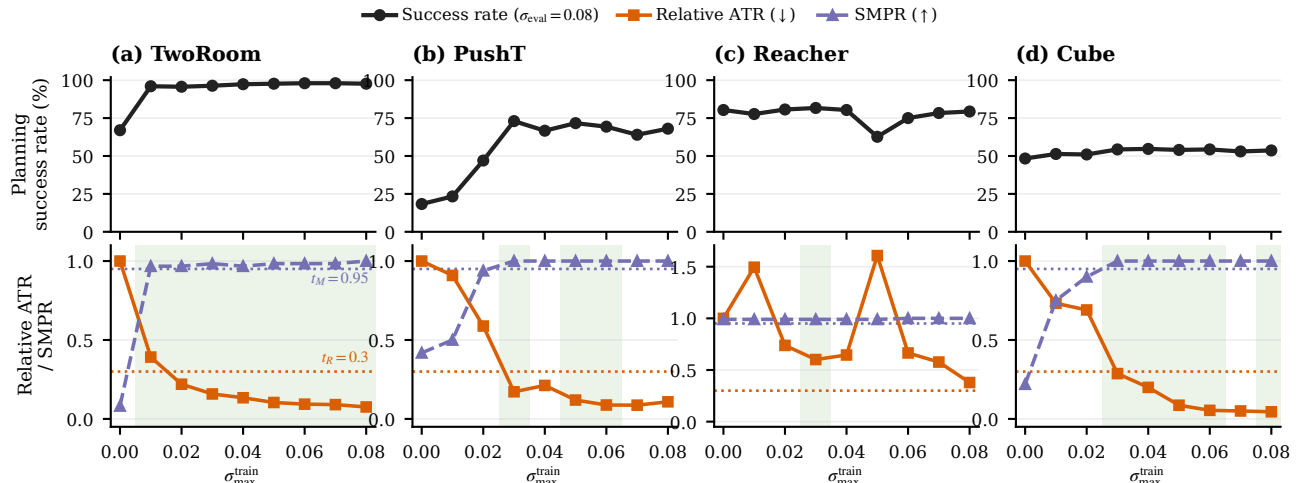
Figure 5: The Figure 2 view repeated on PLDM (one training run per setting), with the same common thresholds drawn as dotted lines; green bands in the diagnostic row mark levels meeting the success-rate criterion. On TwoRoom, PushT, and Cube the relative-ATR curve falls below t_R and SMPR stays above t_M where planning recovers; on Reacher the noisy success rate barely changes across the sweep and relative ATR never clears t_R , so no checkpoint is accepted.
