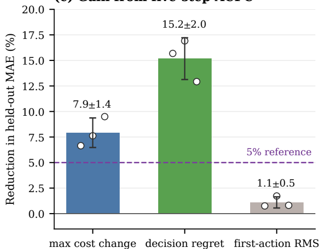
(c) Gain from five-step ACPC
