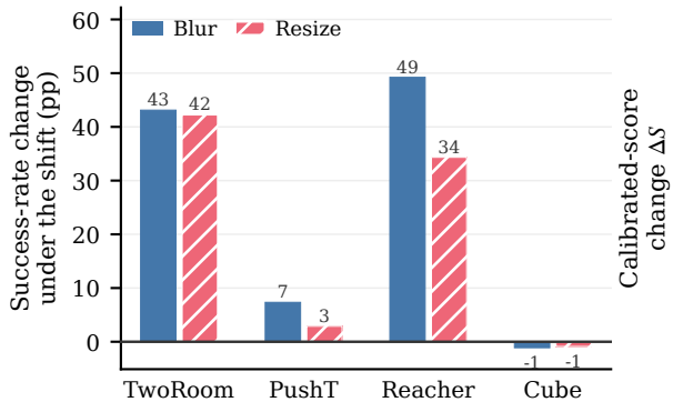
(a) Planning gain
