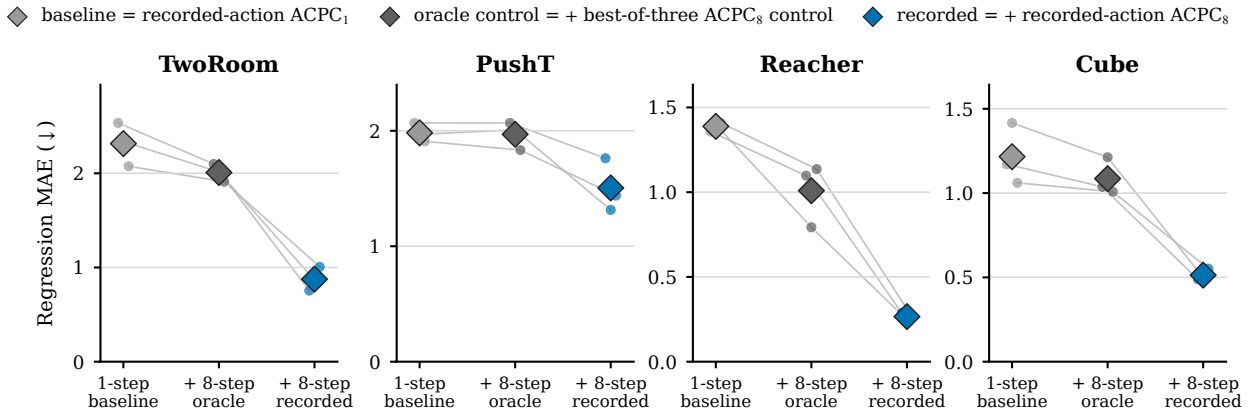
Nested regression feature set (both eight-step models retain the one-step baseline)
