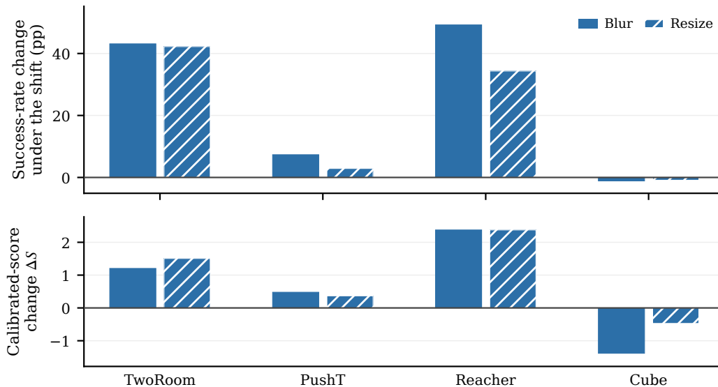
Figure 6: Correspondence between planning gains and the diagnostic under blur and resize. Bars average the three training runs for each task and shift; per-pair values are in Table 10. Top: change in planning success rate from the unaugmented to the \sigma_{\max} = 0.08 checkpoint under the shift. Bottom: change \Delta S in the calibrated score of Equation (17), i.e., how much more margin the noise-trained checkpoint has inside the common thresholds; positive means the diagnostic favors it. Tasks with clear planning gains (TwoRoom, Reacher) also gain score; Cube gains neither.
