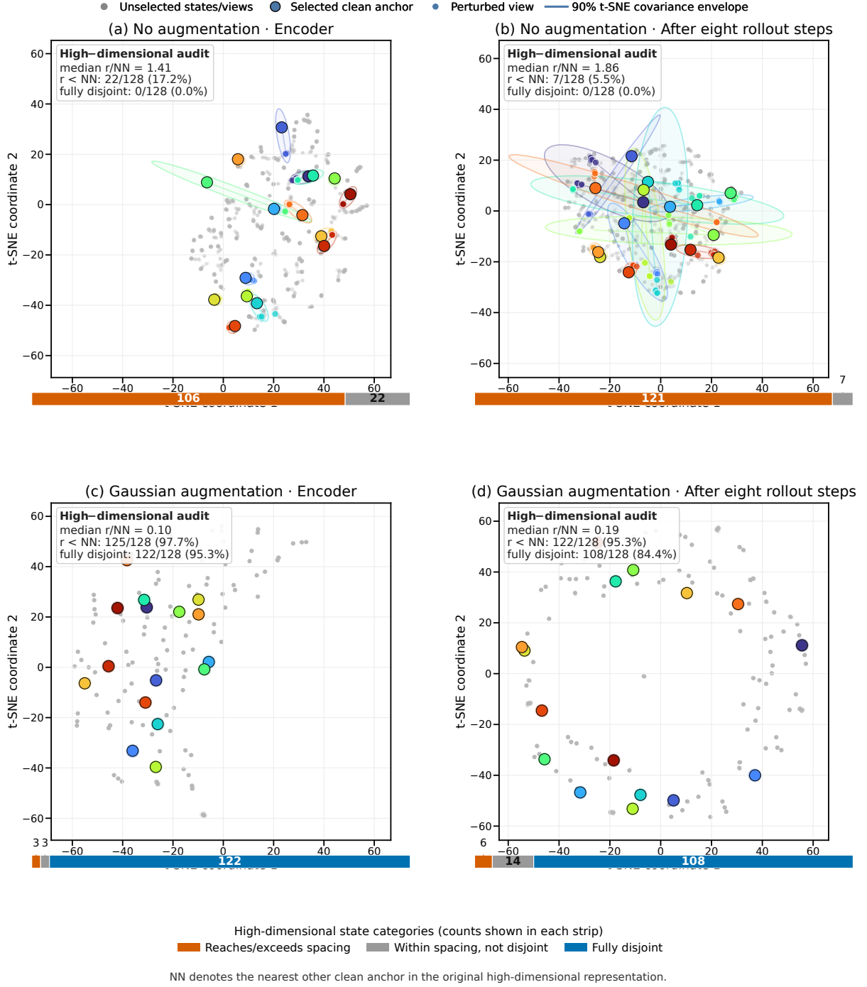
Figure 2: Representative PushT local-geometry audit for LeWM training run 3072. Rows compare the unaugmented and \sigma_{\max} = 0.08 Gaussian-augmented checkpoints; columns show the encoder output and the representation after eight autoregressive rollout steps. Each state has one clean and 18 perturbed views; colors identify a fixed random subset of 16 states, while gray points and all reported statistics cover all 128 states. Each column uses a joint t-SNE fit across the two checkpoints, but t-SNE does not preserve metric geometry: the displayed median r/NN , r < NN counts, and three-category strips are computed in the original high-dimensional representations, not in two dimensions. Reaching nearest-clean spacing is not a semantic-crossover claim, and the 2-D ellipses are only qualitative envelopes. The local view exposes visual spread, but it does not control the neighbor’s task meaning, compare different centers under one shared action sequence, or observe the complete rollout; these limitations motivate ACPC.
