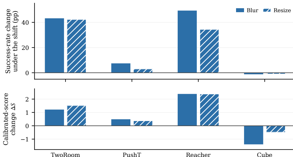
Figure 5: Correspondence between planning gains and the diagnostic under blur and resize. Bars average the three training runs for each task and shift; per-pair values are in Table 10. Top: change in planning success rate from the unaugmented to the \sigma_{\max} = 0.08 checkpoint under the shift. Bottom: change \Delta S in the calibrated score of Equation (17), i.e., how much more margin the noise-trained checkpoint has inside the common thresholds; positive means the diagnostic favors it. Tasks with clear planning gains (TwoRoom, Reacher) also gain score; Cube gains neither.
