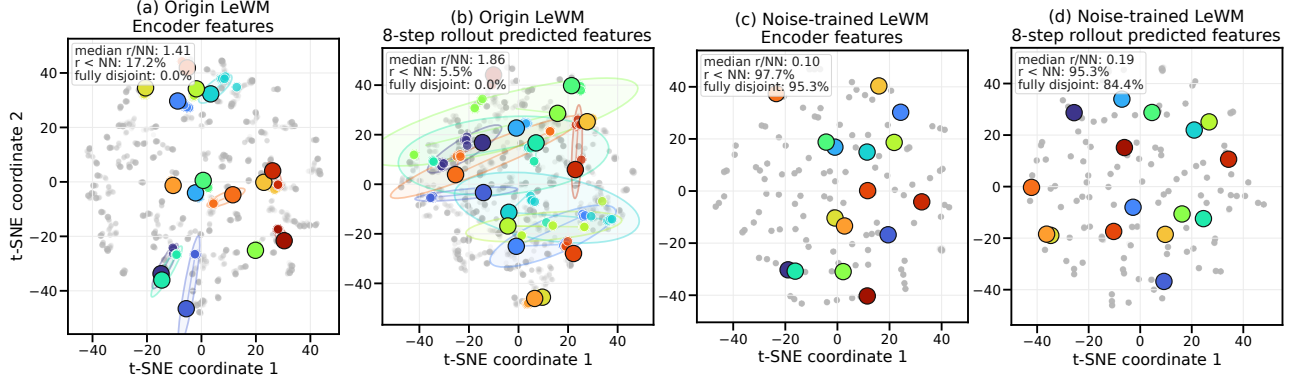
Figure 1: Descriptive local-geometry case study motivating the controlled ACPC comparison. Panels (a)–(d) compare a matched pair of PushT checkpoints—the left two unaugmented, the right two trained with Gaussian augmentation at \sigma_{\max} = 0.08 —at the encoder output and after eight autoregressive rollout steps. Each color denotes one of 16 highlighted histories: the large black-rimmed marker is its clean anchor, smaller same-color markers are its 18 perturbed views, and the faint ellipse is their 90% t-SNE envelope; gray points show all other histories and views. Under strong contraction, smaller markers and ellipses can lie beneath the clean marker. Each panel’s upper-left summary reports, across all 128 anchors, the median r/\text{NN} and the percentages with r < \text{NN} and with fully disjoint high-dimensional enclosing balls. The t-SNE coordinates and ellipses are qualitative and enter none of these metrics.
