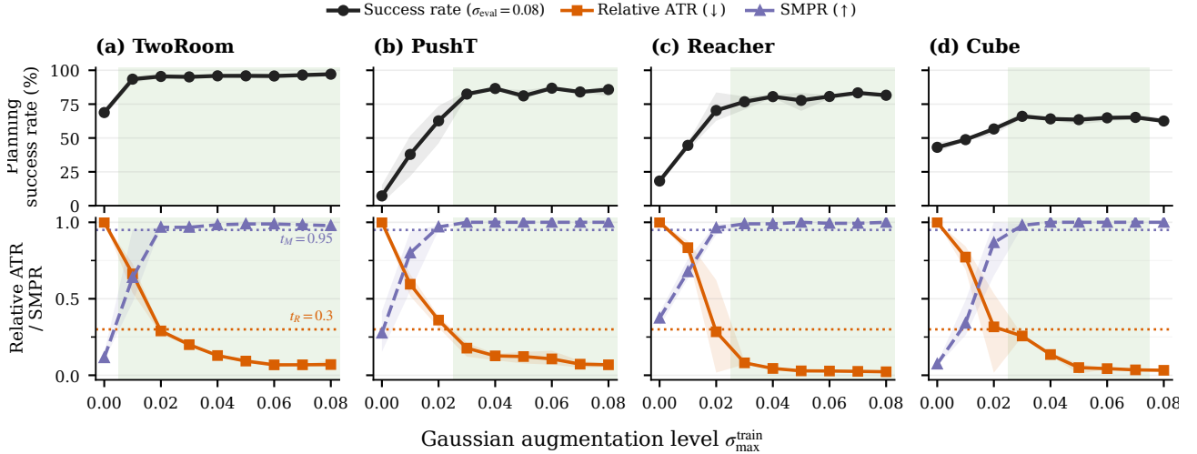
Figure 2: Checkpoint-level planning performance and diagnostics across the complete Gaussian-augmentation sweep. We report planning success rate at evaluation noise \sigma = 0.08 , relative ATR, and SMPR. Lines are across-run means; shaded ranges span the three run means; green bands mark levels meeting the success-rate criterion (Section 4.1) in a majority of runs. Lower ATR (relative to the unaugmented checkpoint) and higher SMPR are favorable. Dotted horizontal lines mark the common thresholds t_R = 0.3 (ATR) and t_M = 0.95 (SMPR) shared across tasks (Section 4.6).
