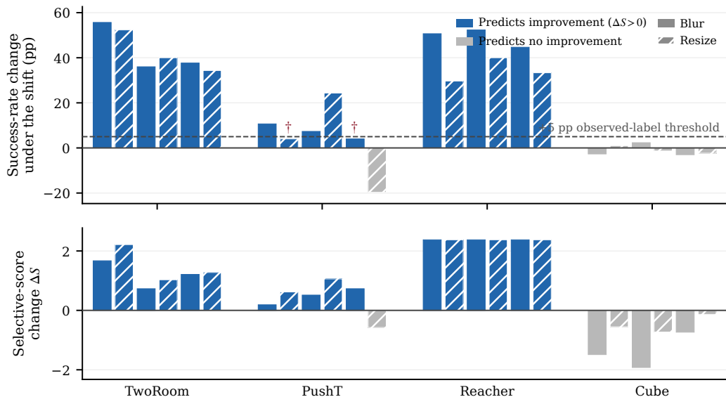
Figure 5: Correspondence between planning gains and the diagnostic under blur and resize for all 24 checkpoint pairs (unaugmented versus \sigma_{\max} = 0.08 ), grouped by task and ordered by training run. Top: success-rate change under the shift; the dashed line is the five-point observed-label threshold, and daggers mark the two discordant pairs, both at +4 points. Bottom: selective-score change \Delta S of the same pairs under the common thresholds. Bar color gives the diagnostic verdict; hatched bars are resize. The label’s clean-loss condition changes no label among these pairs.
