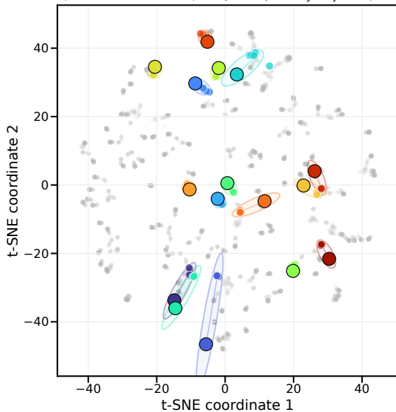
Noise-trained LeWM: Encoder features
