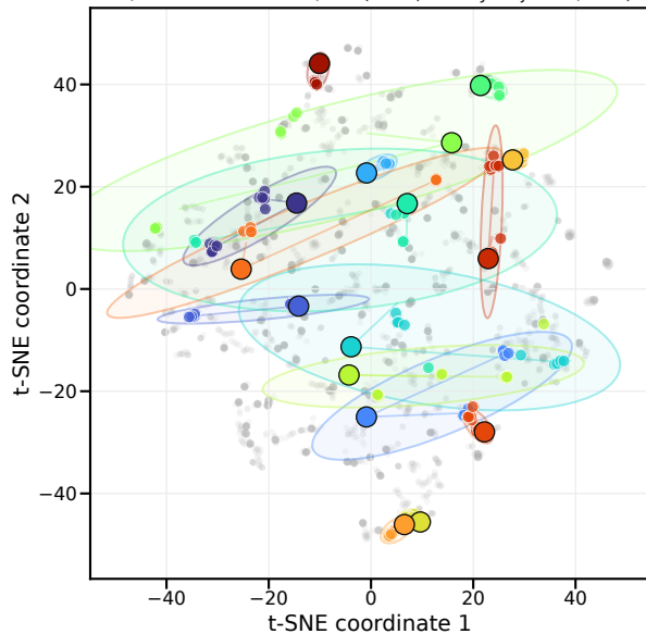
Noise-trained LeWM: 8-step rollout predicted features
