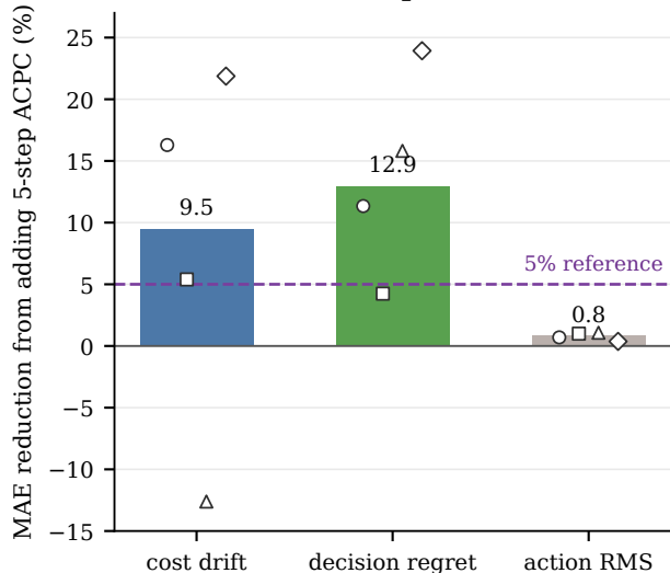
(c) Cross-task 5-step increment
