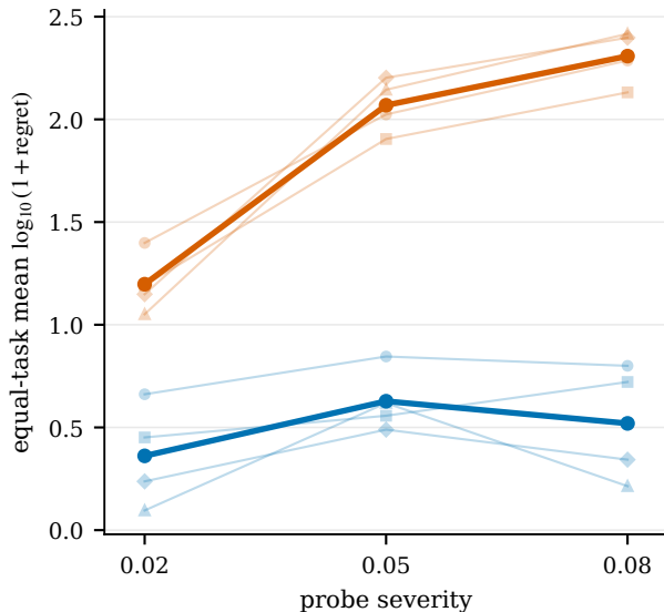
(b) Adaptive-CEM decision regret
