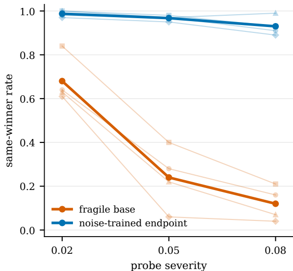
(a) Fixed-pool top-1 stability
