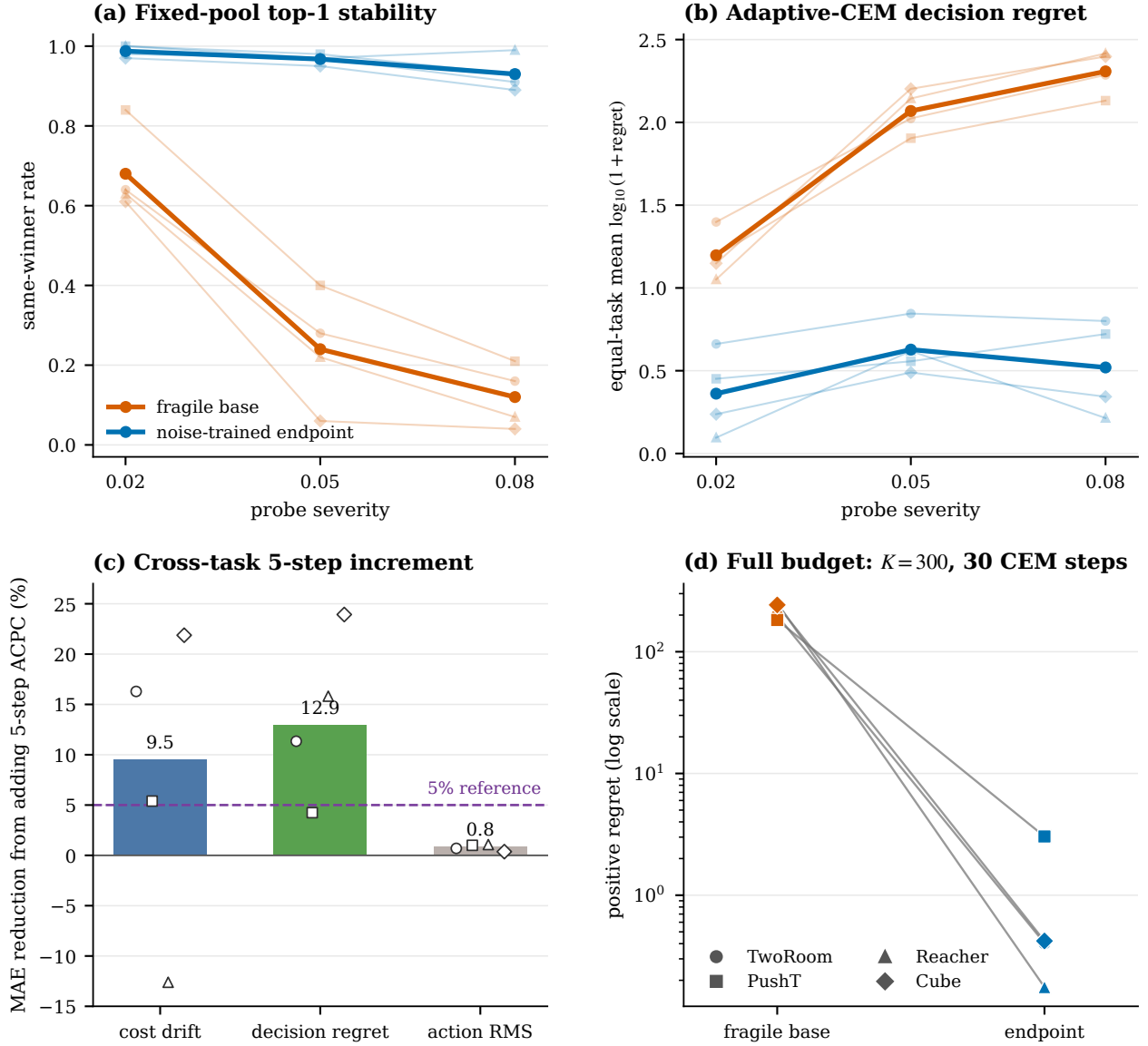
Figure 4: Planner-aligned ACPC evidence. Faint curves/points show tasks and heavy curves show equal-task means. Panels (a)–(c) use 100 histories per task and checkpoint role: (a) same-winner frequency for the shared fixed pool, (b) adaptive-CEM regret of the perturbed decision when rescored on the clean history, and (c) the prediction-error reduction from adding candidate-conditioned five-step ACPC beyond severity, checkpoint role, one-step ACPC, and nominal margin. Panel (d) reports the same regret outcome on 16 histories at the deployed K = 300 , 30-step budget. These are behavior-blind planner diagnostics, not closed-loop return.
