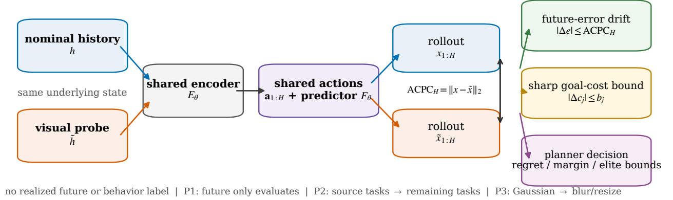
Figure 1: ACPC compares two views of the same state under one shared action sequence. The paired rollout difference is target-free at scoring time, yet it controls error drift to any common future and, for LeWM’s goal cost, yields candidate-wise cost and planner-margin certificates. Adaptive-CEM implications are conditional on aligned pools and certified elite sets at every iteration.
