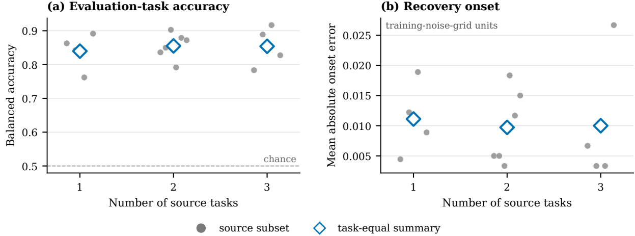
Figure 5: Cross-task portability over every source/evaluation partition. For each source subset, ATR and SMPR thresholds are selected using only those tasks and then applied unchanged to all remaining tasks. Small points are individual source subsets; large points give task-equal summaries. Adding source tasks is not monotonically beneficial because composition matters, but the aggregate rule remains stable across one-, two-, and three-task sources.
