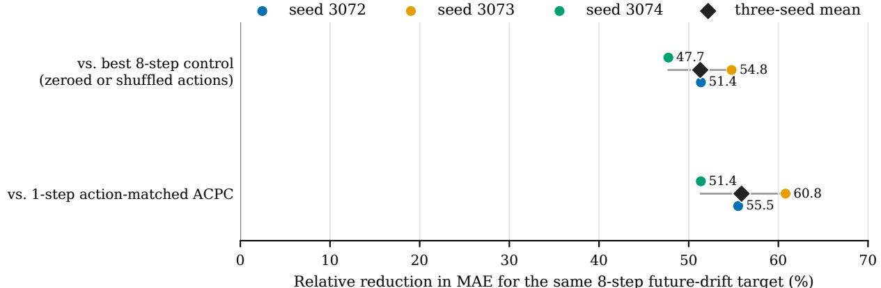
Figure 3: Recorded-action eight-step ACPC adds information about a common eight-step future-drift target. Points are equal-task MAE reductions for three independently trained models; diamonds are their means. The upper comparison holds rollout horizon fixed and changes only action structure, so the result cannot be explained by longer rollouts mechanically accumulating more error. Each seed improves on all four tasks.
