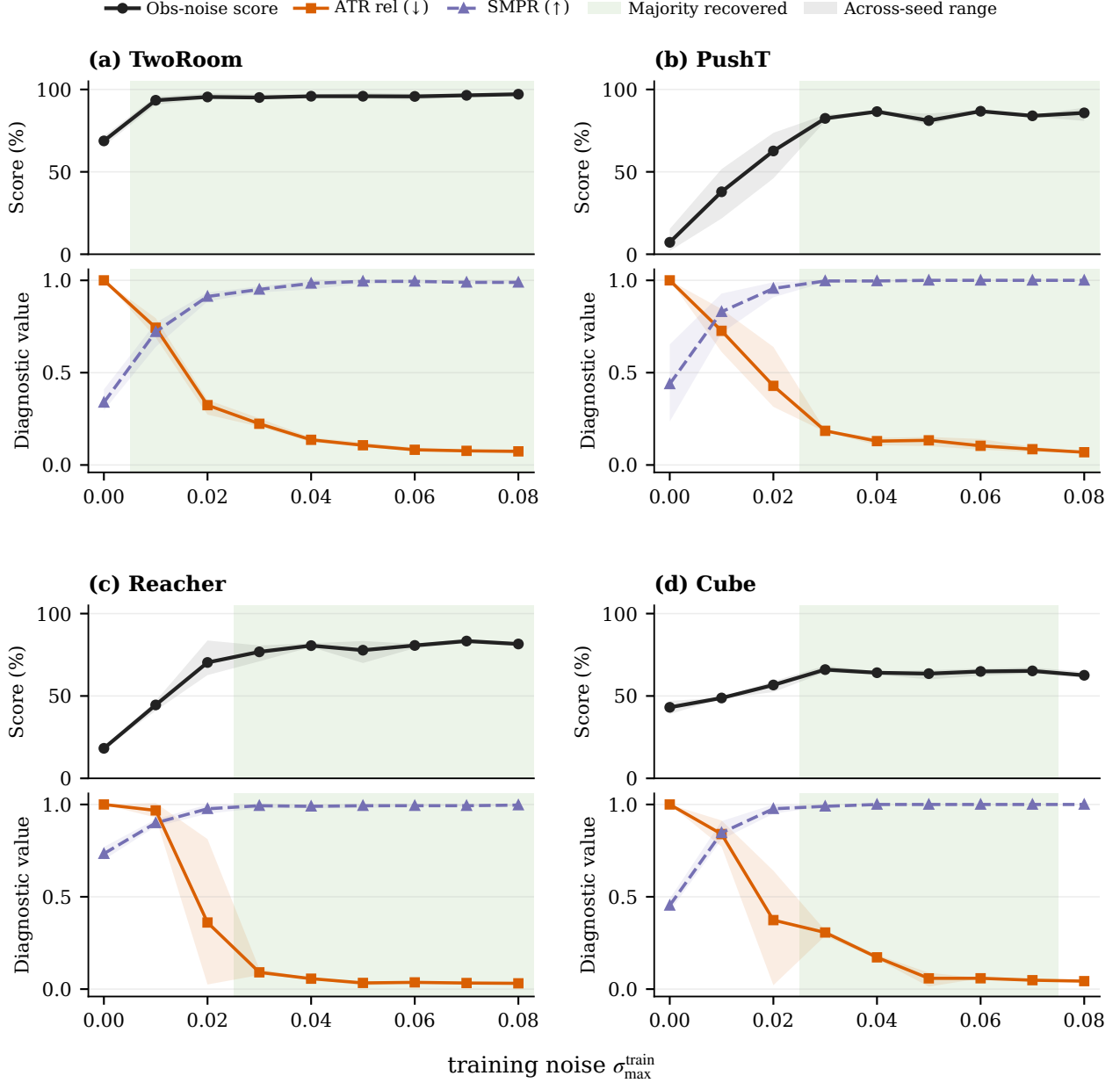
Figure 2: Closed-loop success under observation noise and the two diagnostic components across the complete Gaussian training sweep. Solid lines first average evaluation replicates within each training seed and then average seeds 3072/3073/3074; translucent envelopes span the three seed means. ATR is divided by the corresponding task \times seed no-noise value for display (base = 1); SMPR remains on its original rate scale. Green bands require at least 80% of the attainable stressed-score gain, at most a five-point clean loss, and recovery in a majority of seeds. Lower ATR and higher SMPR co-move with recovery on all four tasks, but this descriptive alignment alone does not establish action or semantic specificity.
