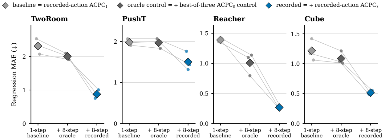
Figure 3: Cross-validated MAE for predicting the error drift d on the unaugmented checkpoints; lower is better. Each model is evaluated on trajectory groups excluded from fitting. Small points are training runs, thin lines join the same run, and diamonds are task means. The in-figure legend labels correspond to Base, Base+Control 8 , and Base+ACPC 8 as defined in Section 4.4. Base+ACPC 8 is lowest in all 12 task–run cells; latent-error scales are task-specific, so compare within a panel.
