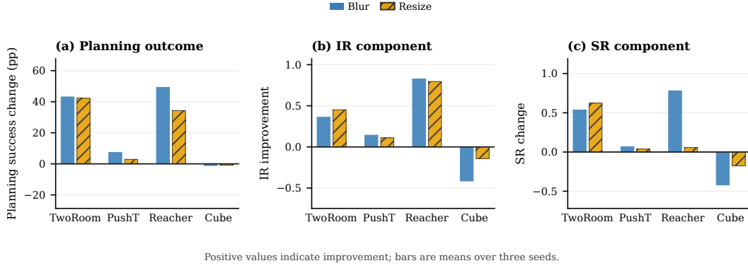
Figure 8: Changes from the unaugmented checkpoint to the checkpoint trained at \sigma_{\max} = 0.08 under blur and resize. Panels show (a) planning-success change in percentage points, (b) IR improvement 1 - \text{IR}_q^{\text{rel}} , and (c) SR change. Bars are means across three training runs, and positive values indicate improvement.
