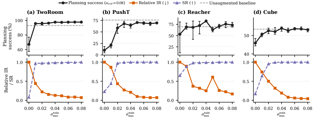
Figure 7: Complete PLDM Gaussian-noise training sweep over three runs. Curves show three-run means and success bars span the across-run range. The summary in Table 1 includes every augmented level rather than selecting a recovery subset.
