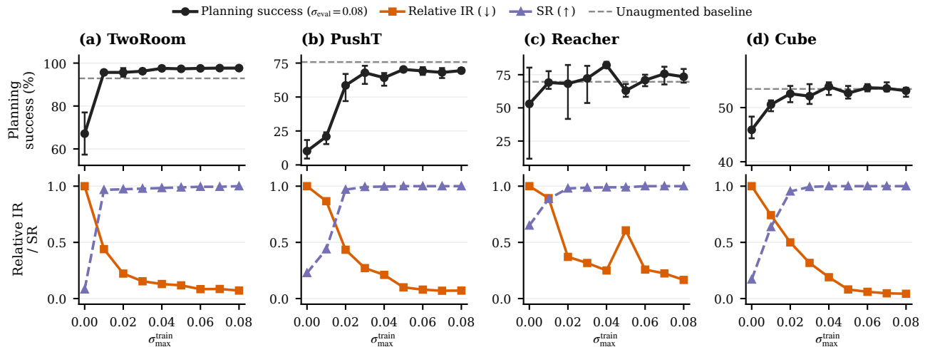
Figure 7: PLDM Gaussian-noise training sweep over three independent training runs. Curves show run means, and success-rate error bars span the run range. The dashed gray line marks clean success of the unaugmented checkpoint, and the leftmost black point is its success at evaluation noise \sigma = 0.08 . Relative IR equals one at that checkpoint. Across tasks, stronger augmentation generally lowers relative IR and raises SR, while planning success under evaluation noise also generally improves from the unaugmented checkpoint.
