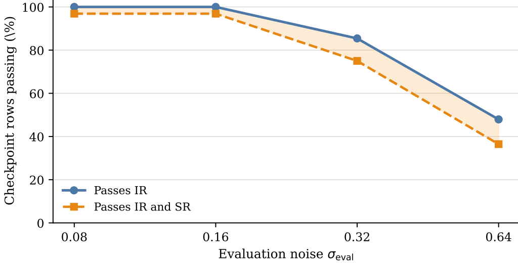
Figure 4: IR and SR become restrictive at different evaluation severities. Both curves use the same denominator of 96 task-training-run-training-strength rows ( 4 \times 3 \times 8 ) at each severity. The blue curve counts rows passing IR; the orange curve counts rows passing both conditions, and the shaded gap is the additional SR veto. The IR-pass counts are 96, 96, 82, and 46 as \sigma_{\text{eval}} increases; SR vetoes 3, 3, 10, and 11 of those rows, leaving 93, 93, 72, and 35 joint passes. Counts are descriptive: the same checkpoints recur across severity slices, so the points are not independent; the task breakdown is in Appendix D. This decomposition shows when each condition is active; it does not measure checkpoint-selection accuracy.
