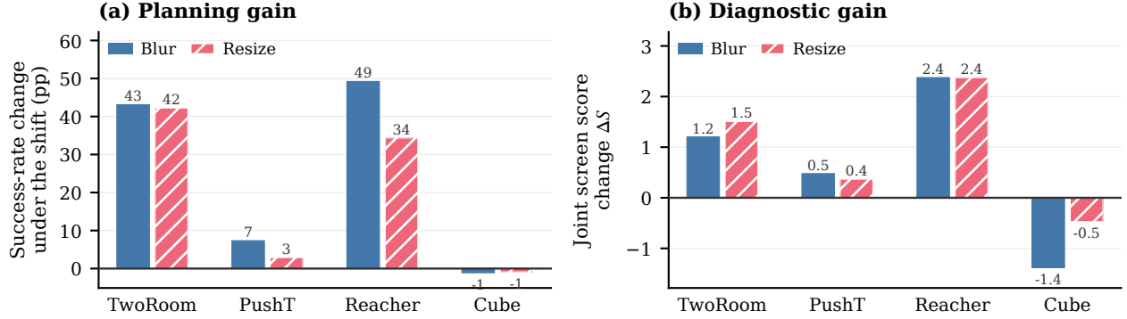
Figure 8: Relative checkpoint comparison under blur and resize. Bars average the three training runs for each task and shift; per-pair values are in Table 9. Panel (a) shows the change in planning success from the unaugmented to the \sigma_{\max} = 0.08 checkpoint. Panel (b) shows the change in the IR–SR score of Equation (12); positive favors the augmented checkpoint but is not an absolute pass decision.
