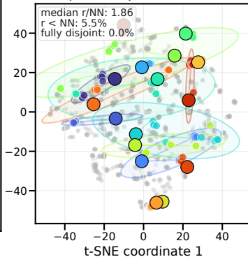
(b) Origin LeWM 8-step rollout predicted features
