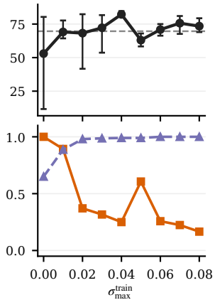
(c) Reacher
