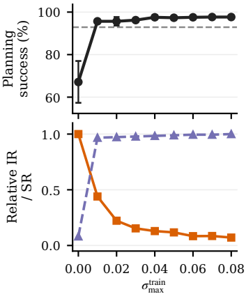
(a) TwoRoom
