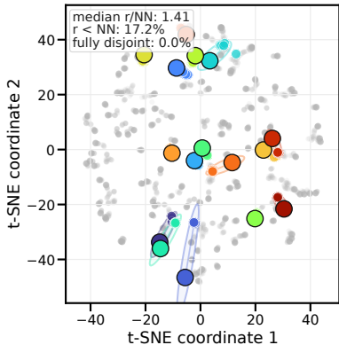
Origin LeWM Encoder features
