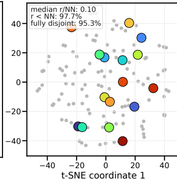
Noise-trained LeWM Encoder features
