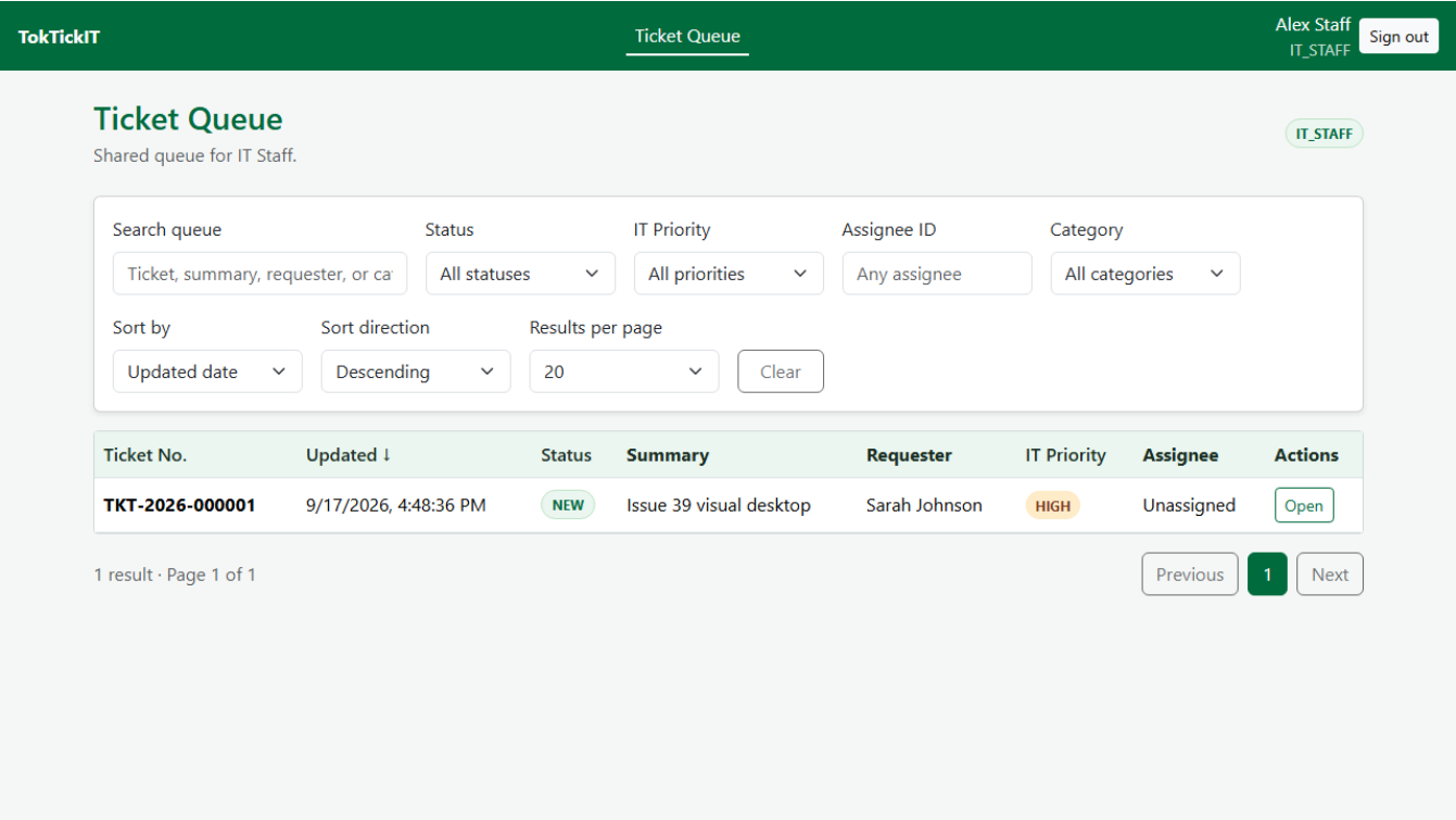
Figure 9.4. Staff Queue — desktop
