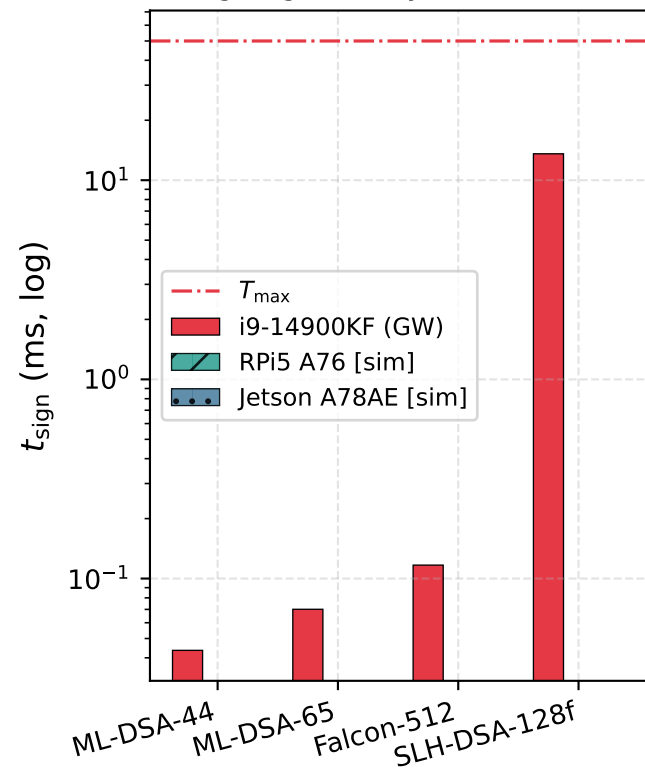
(a) Signing Latency — All Platforms
