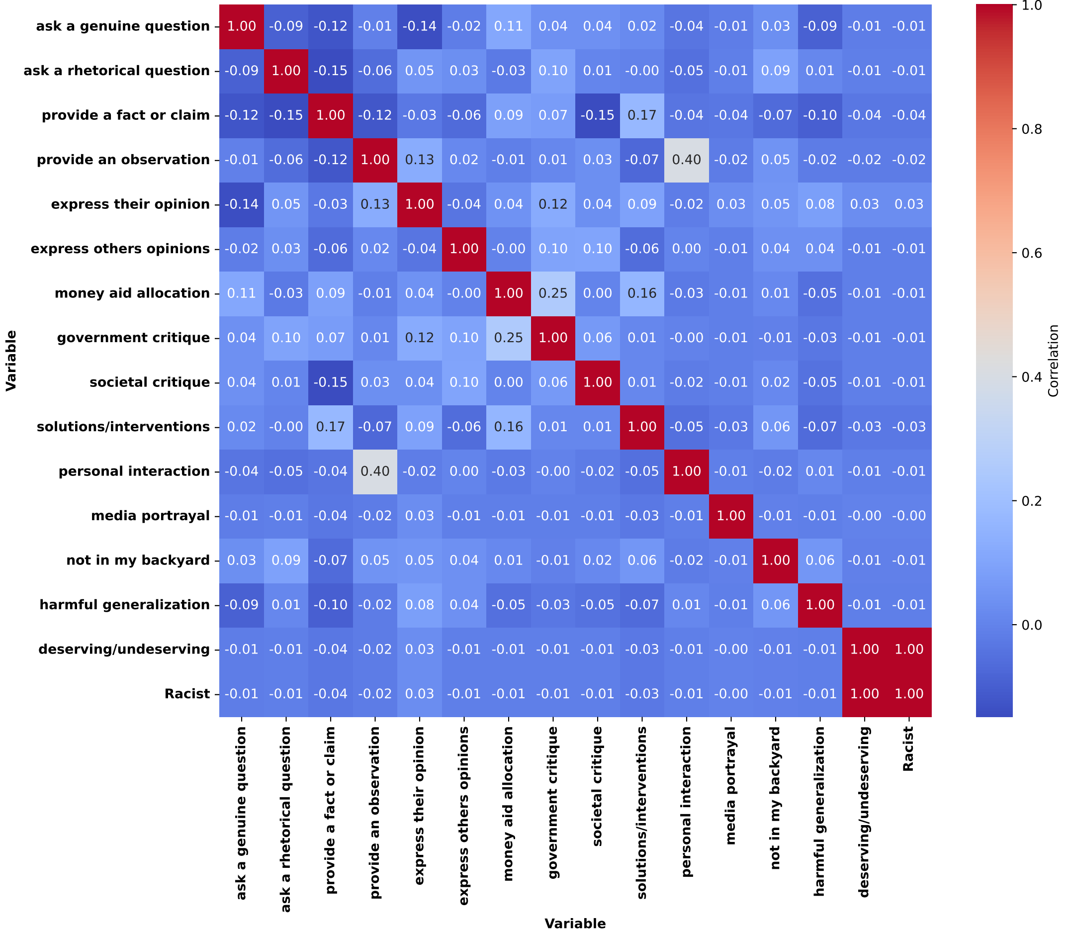
Correlation Matrix of Soft Label Variables (0.5 as 0)
