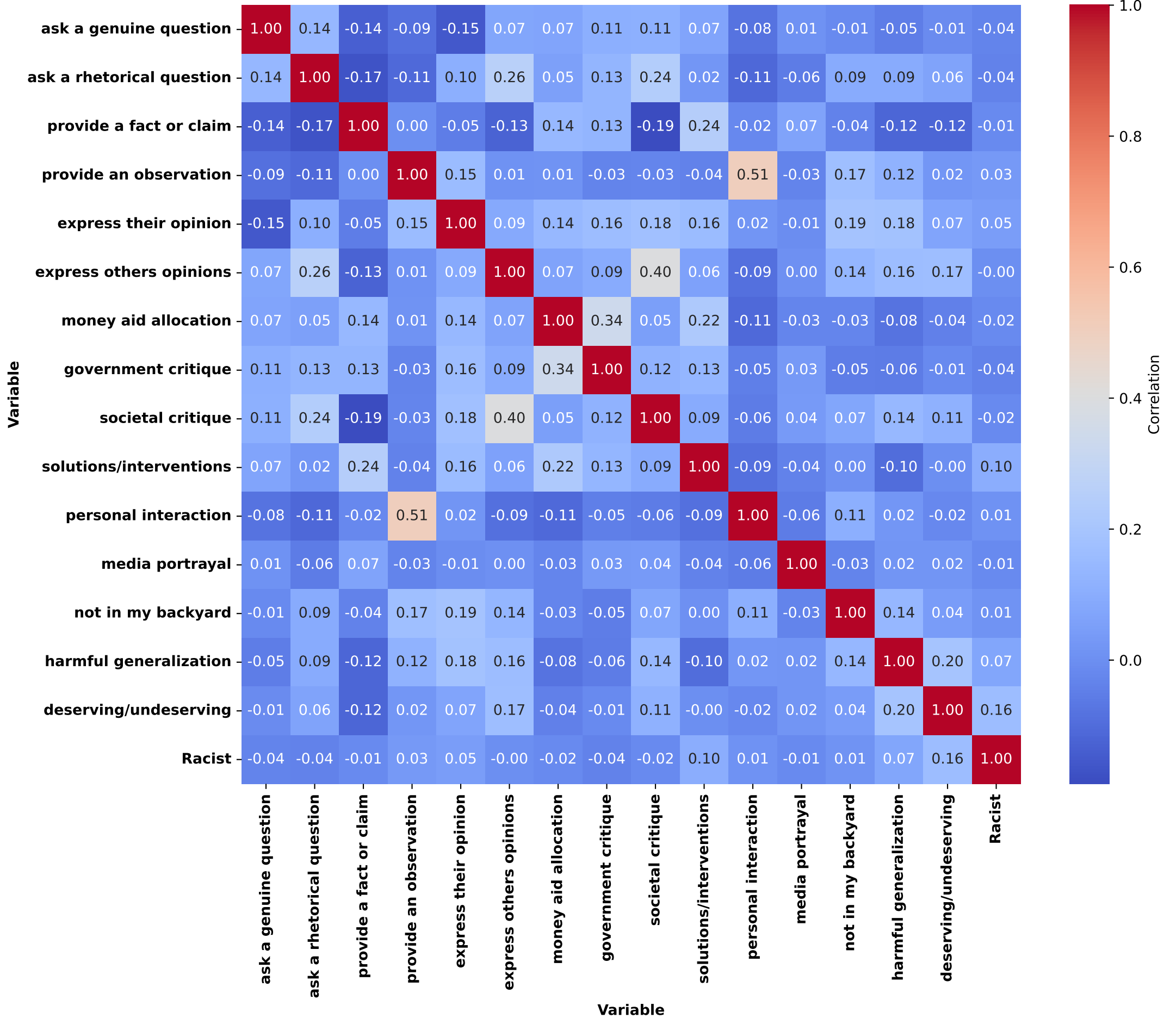
Correlation Matrix of Gold Standard Annotation Variables
