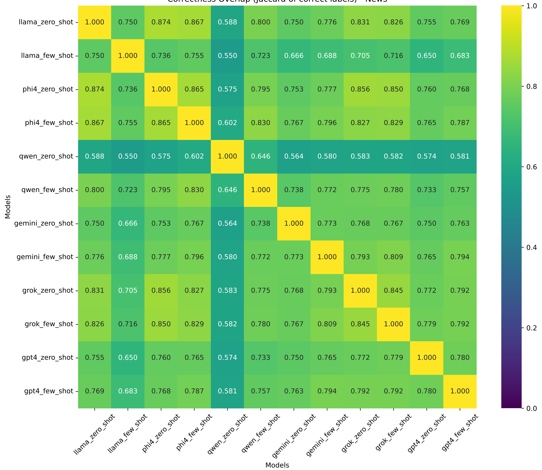
Correctness Overlap (Jaccard of correct labels) - News
