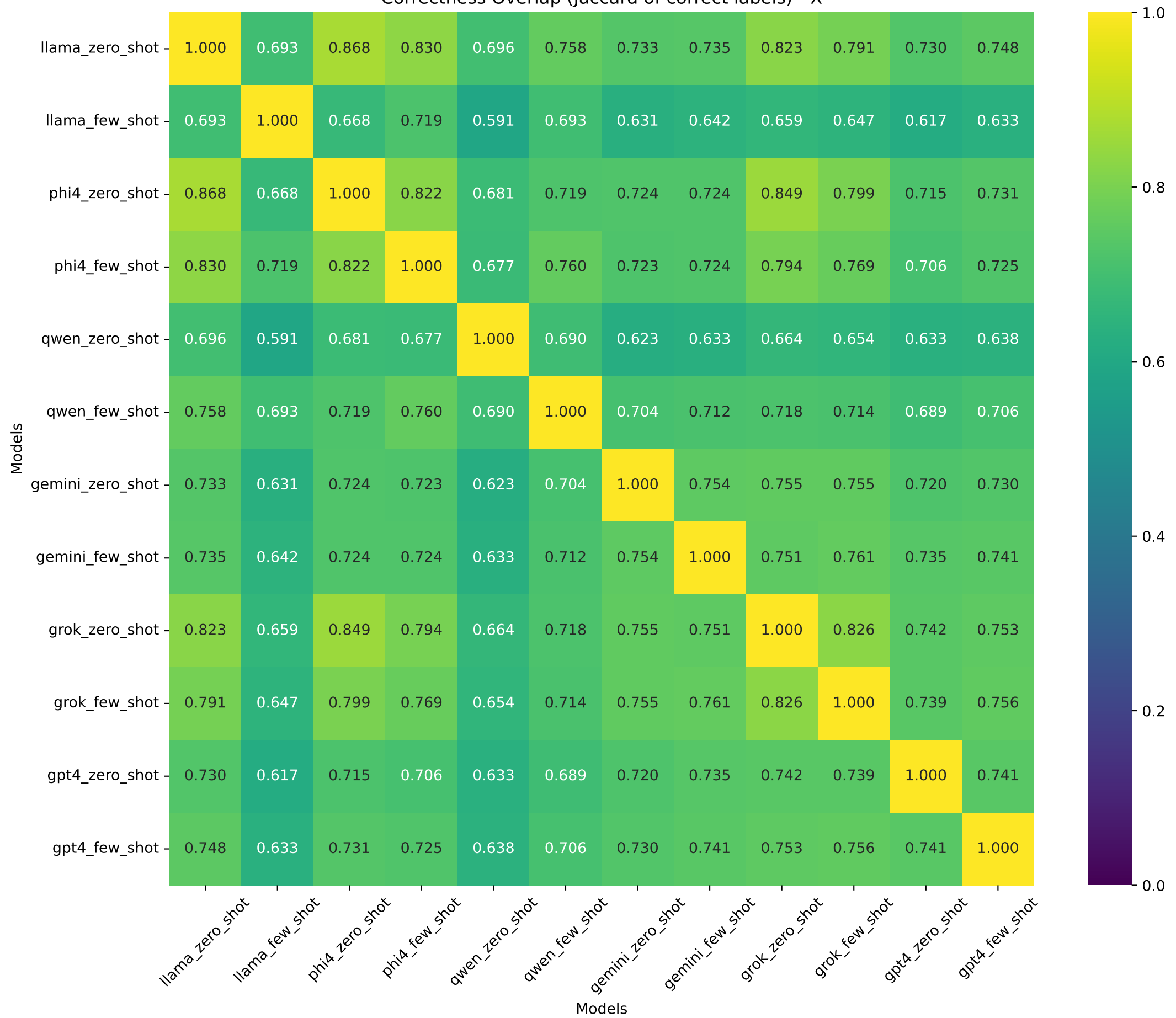
Correctness Overlap (Jaccard of correct labels) - X
