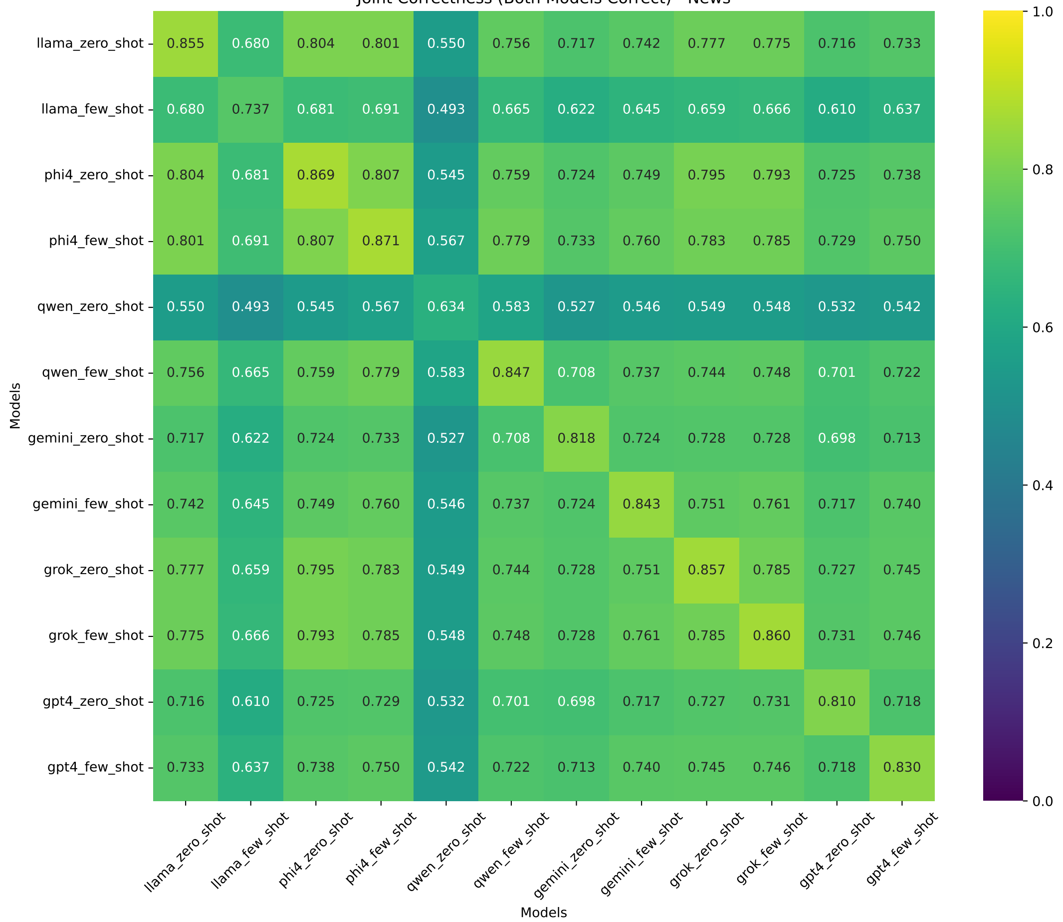
Joint Correctness (Both Models Correct) - News
