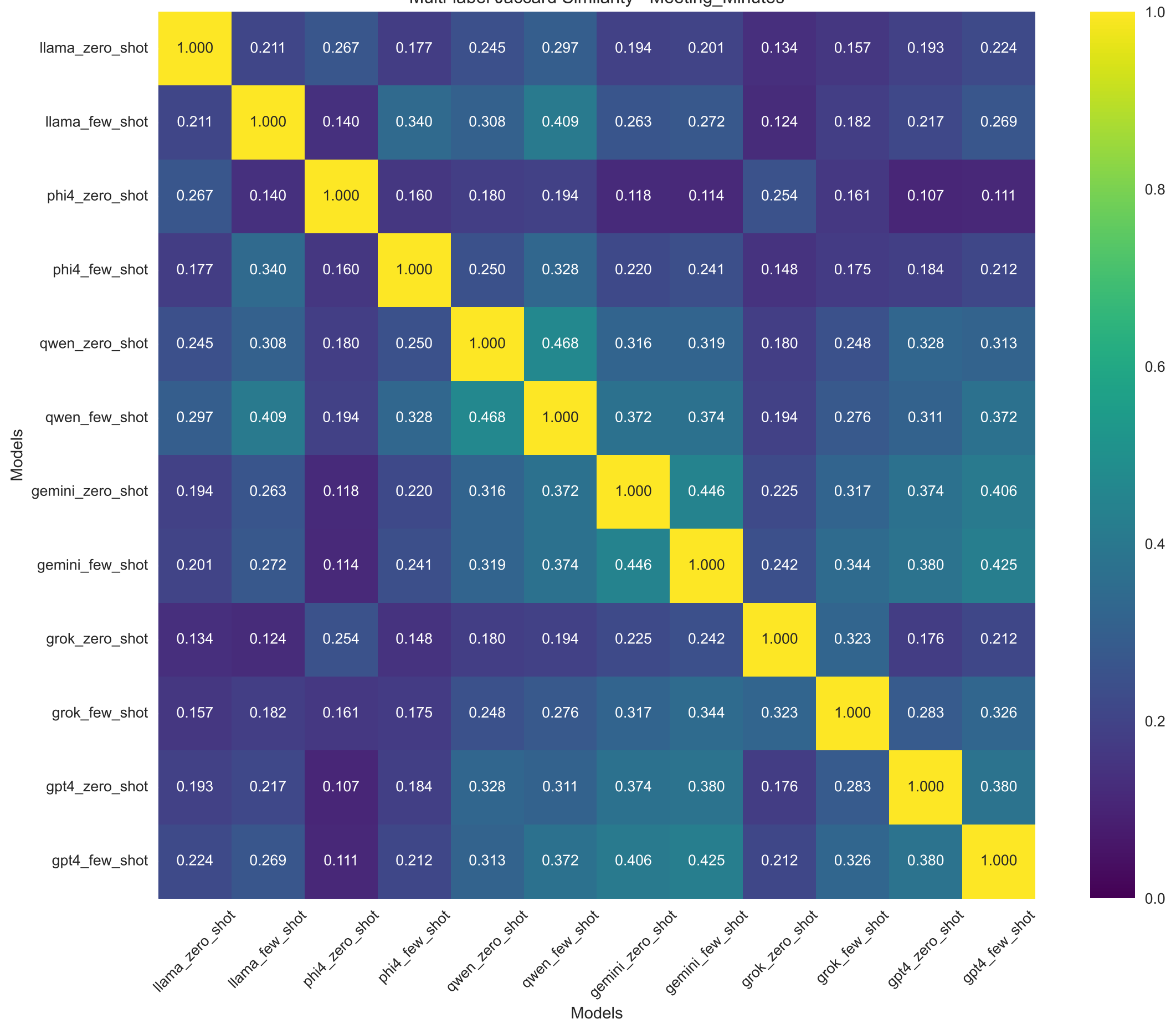
Multi-label Jaccard Similarity - Meeting_Minutes
