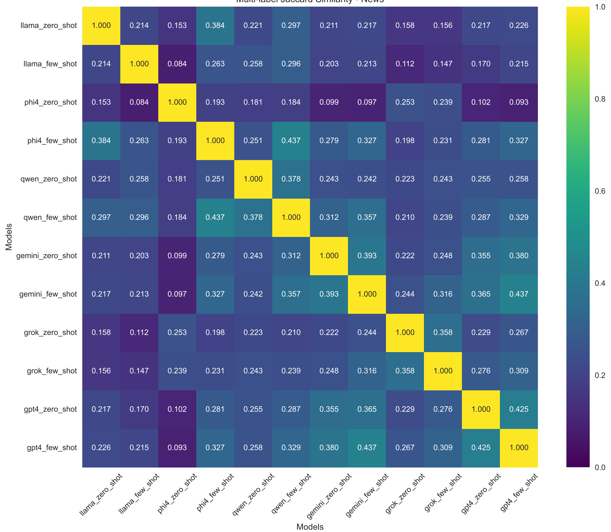
Multi-label Jaccard Similarity - News
