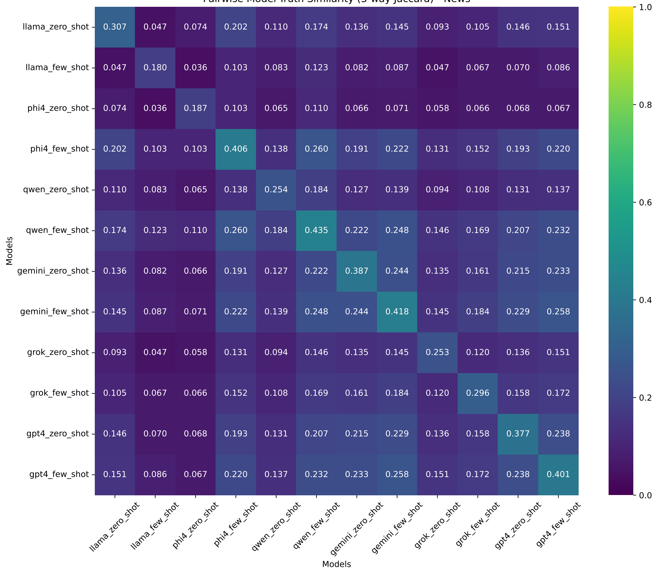
Pairwise Model-Truth Similarity (3-way Jaccard) - News
