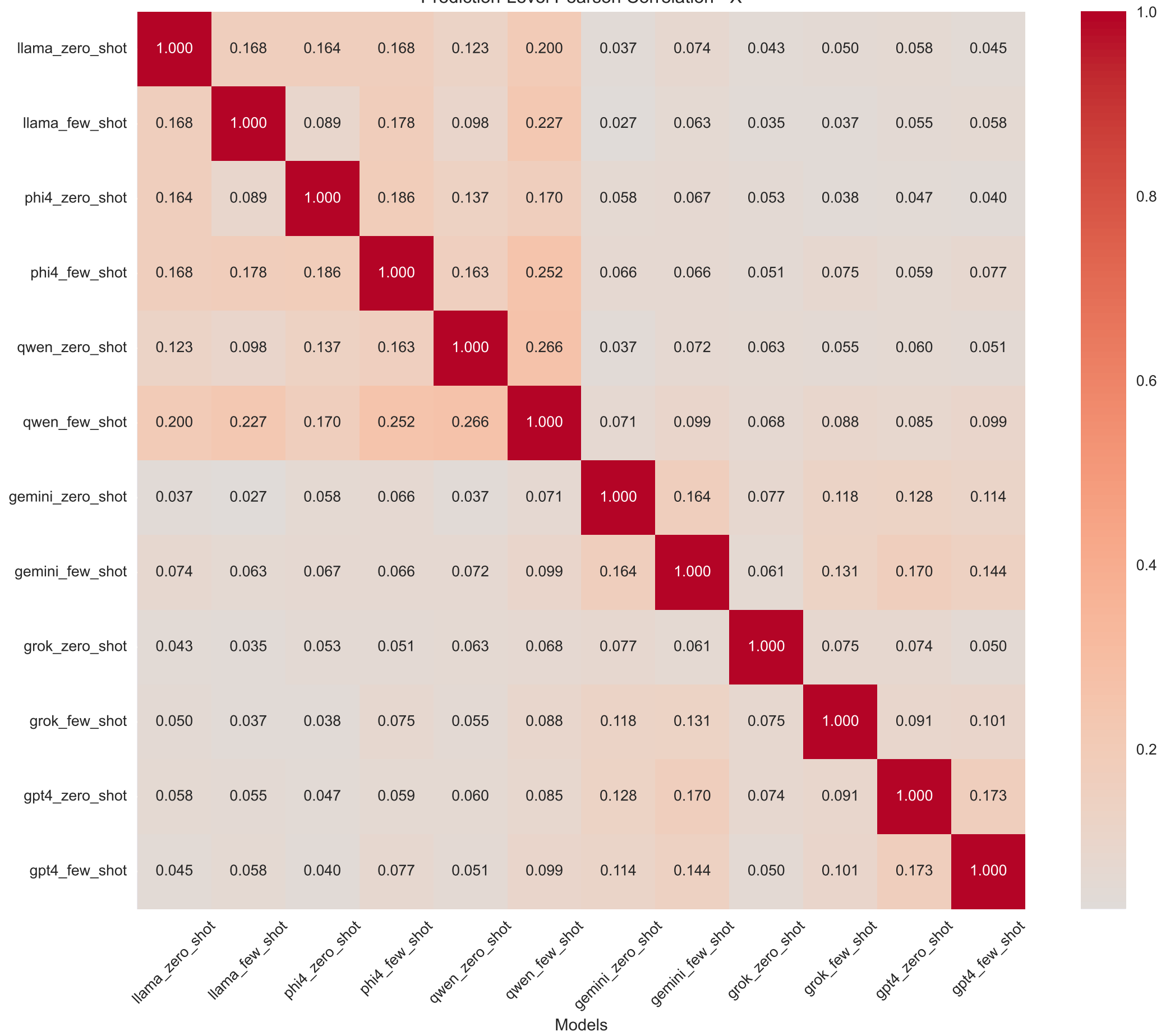
Prediction-Level Pearson Correlation - X
