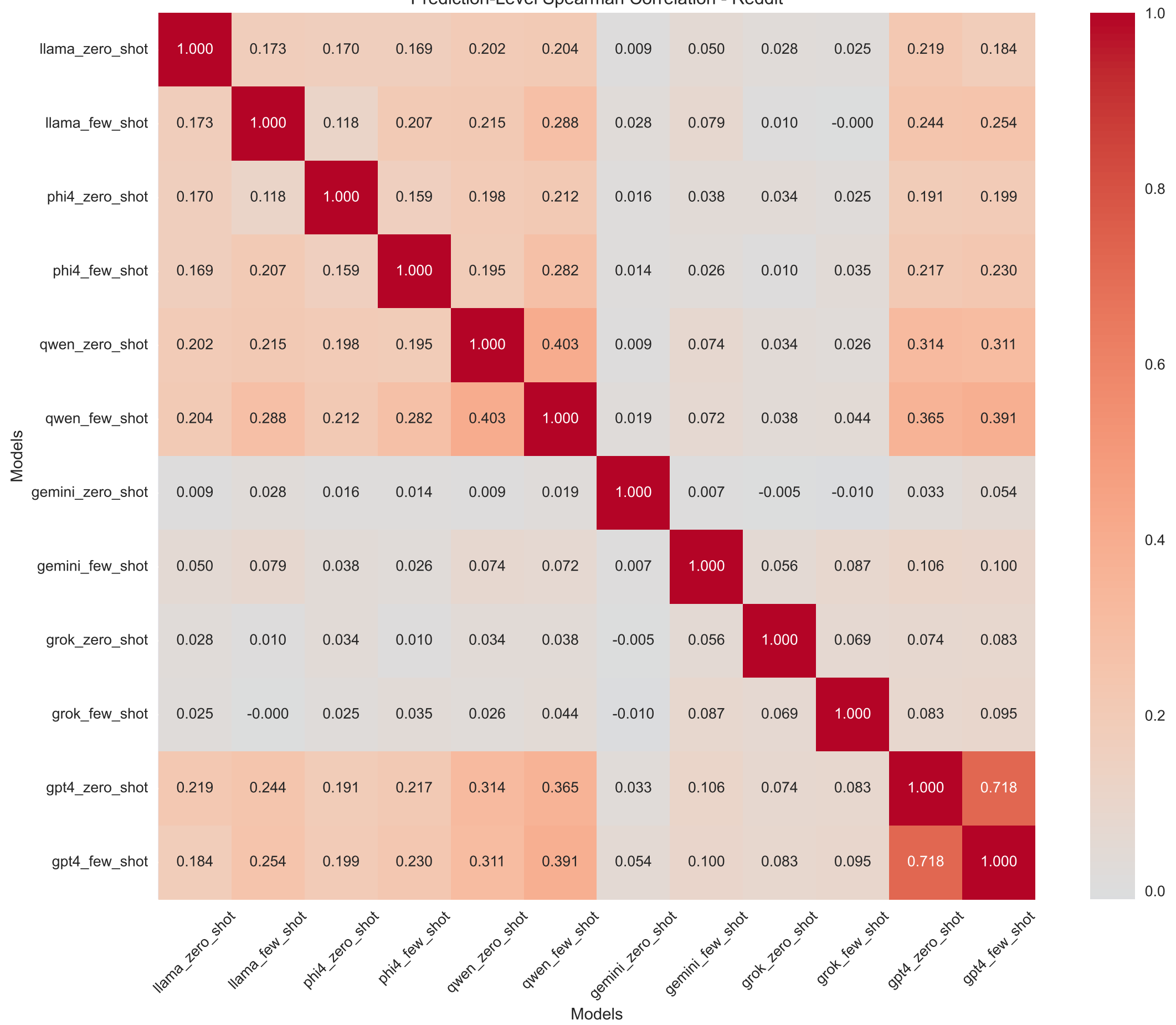
Prediction-Level Spearman Correlation - Reddit
