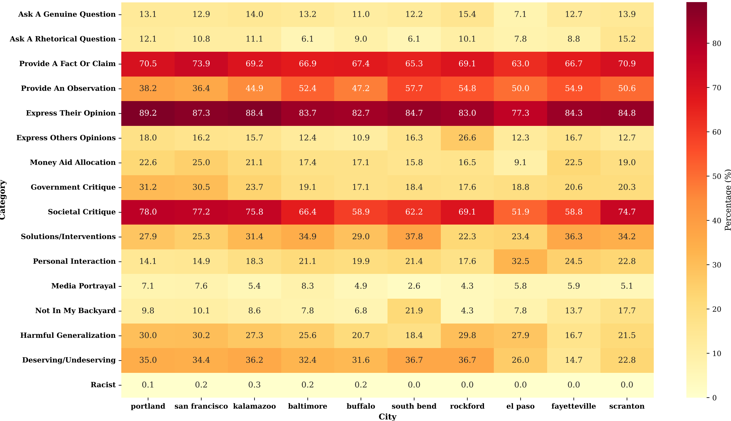
Reddit Classification Categories Heatmap by City
