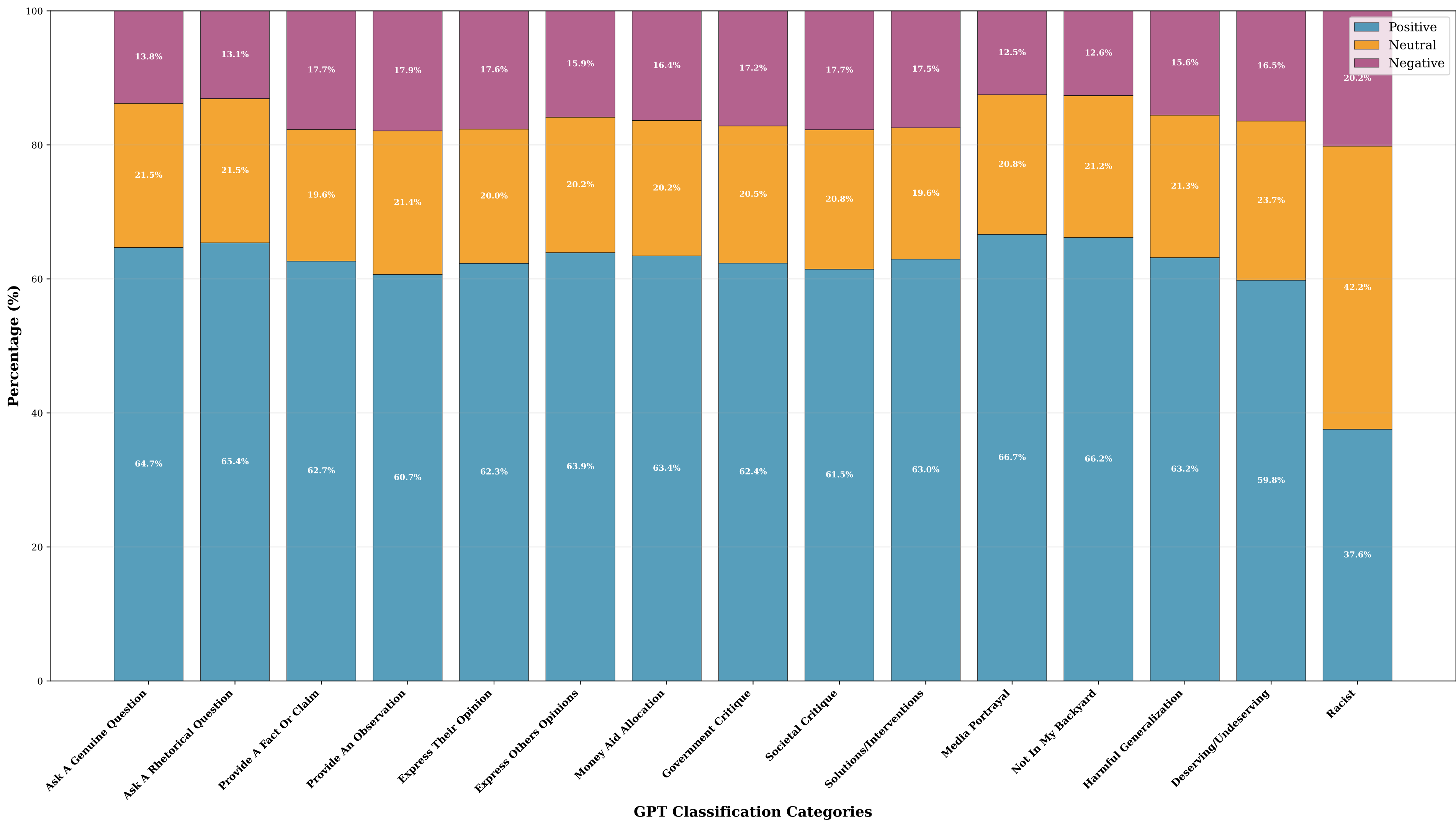
Sentiment Distribution Across GPT Classification Categories (All Data Sources Combined)
