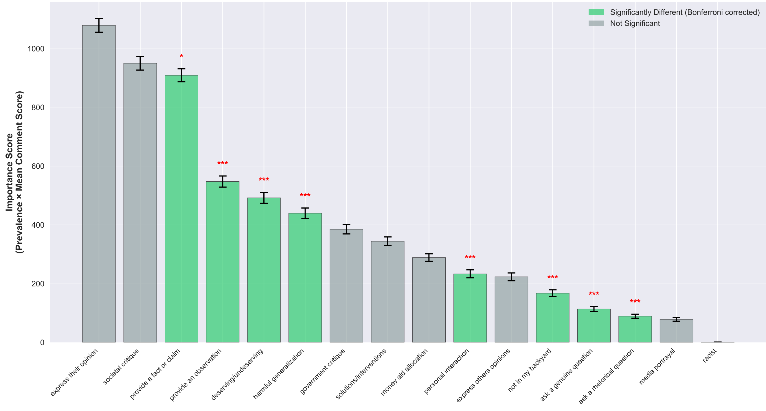
Category Importance on Reddit (All 16 Categories) Error bars = Standard Error, * p<0.05, ** p<0.01, *** p<0.001 (Bonferroni corrected)
