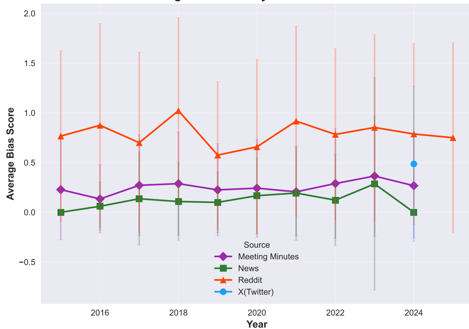
Average Bias Score by Year - Small Cities
