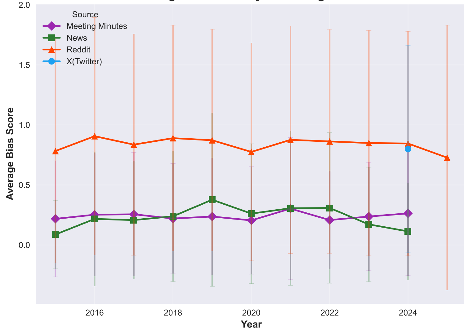
Average Bias Score by Year - Large Cities
