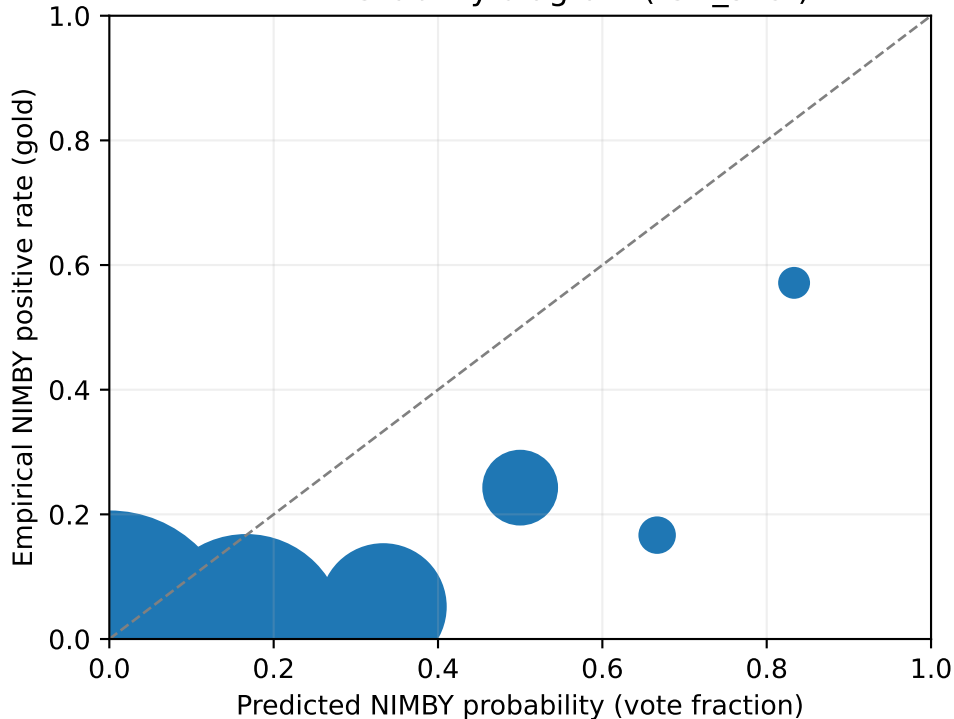
NIMBY reliability diagram (few_shot)
