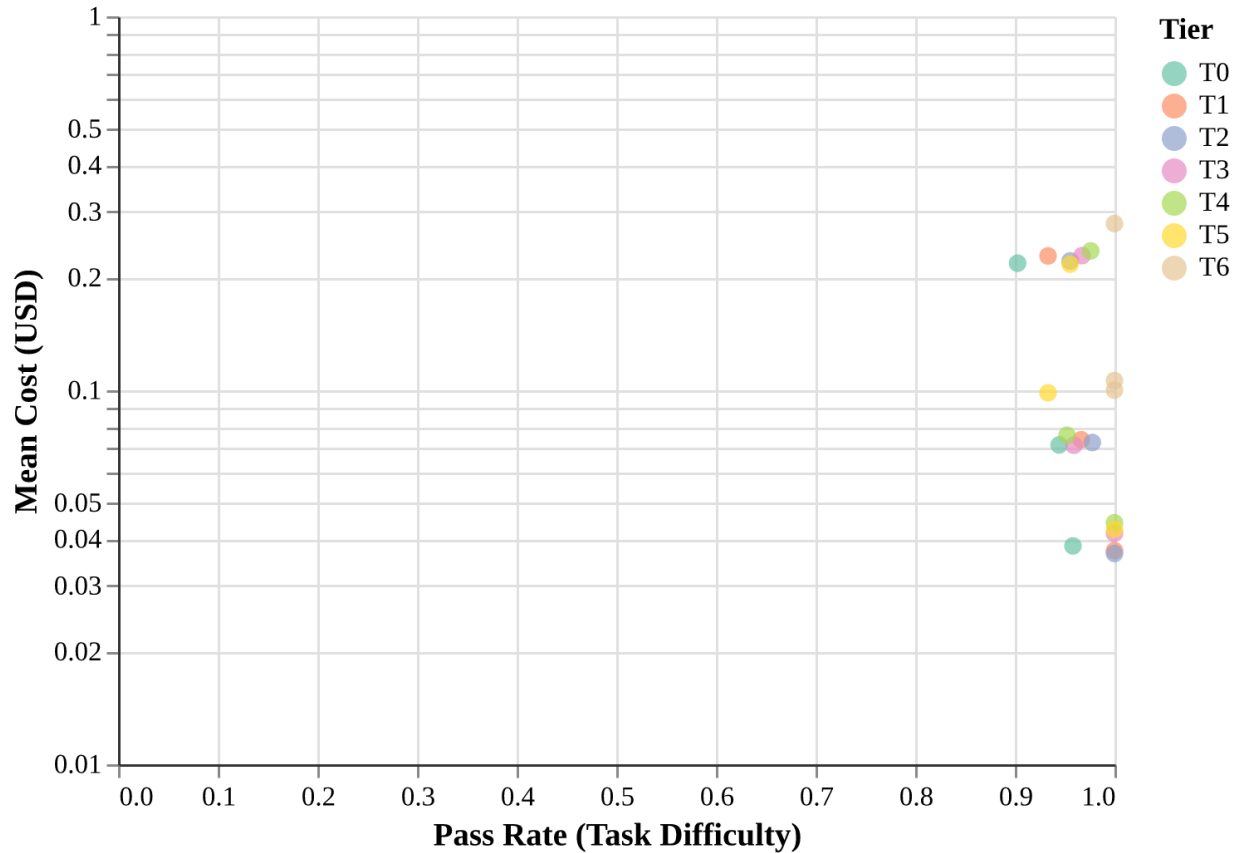
Figure 10: Cost scaling across experiments. Cost is driven primarily by task characteristics—repository size, language complexity, and required context—rather than architectural tier. The spread within each experiment reflects run-to-run variance, not tier differences.
