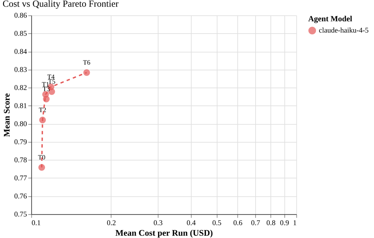
Figure 11: Cost–quality Pareto frontier. Each point represents a tier (aggregated across experiments), plotted by mean cost per run ( x -axis, log scale) and mean consensus score ( y -axis). Pareto-optimal points lie on the upper-left frontier. The narrow spread of points reflects the overall high pass rate (0.966) and cost invariance across tiers.
