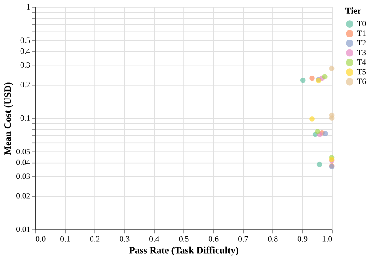
Figure 10: Cost scaling across experiments. Cost is driven primarily by task characteristics—repository size, language complexity, and required context—rather than architectural tier. The spread within each experiment reflects run-to-run variance, not tier differences.
