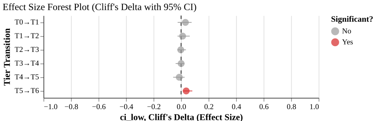
Figure 5: Forest plot of Cliff’s \delta effect sizes for pairwise tier comparisons on score (lower-numbered tier is reference group; negative \delta indicates the higher-numbered tier has lower scores). Effect sizes are uniformly small, consistent with the non-significant omnibus test on pass rate. Error bars show 95% bootstrap confidence intervals.
