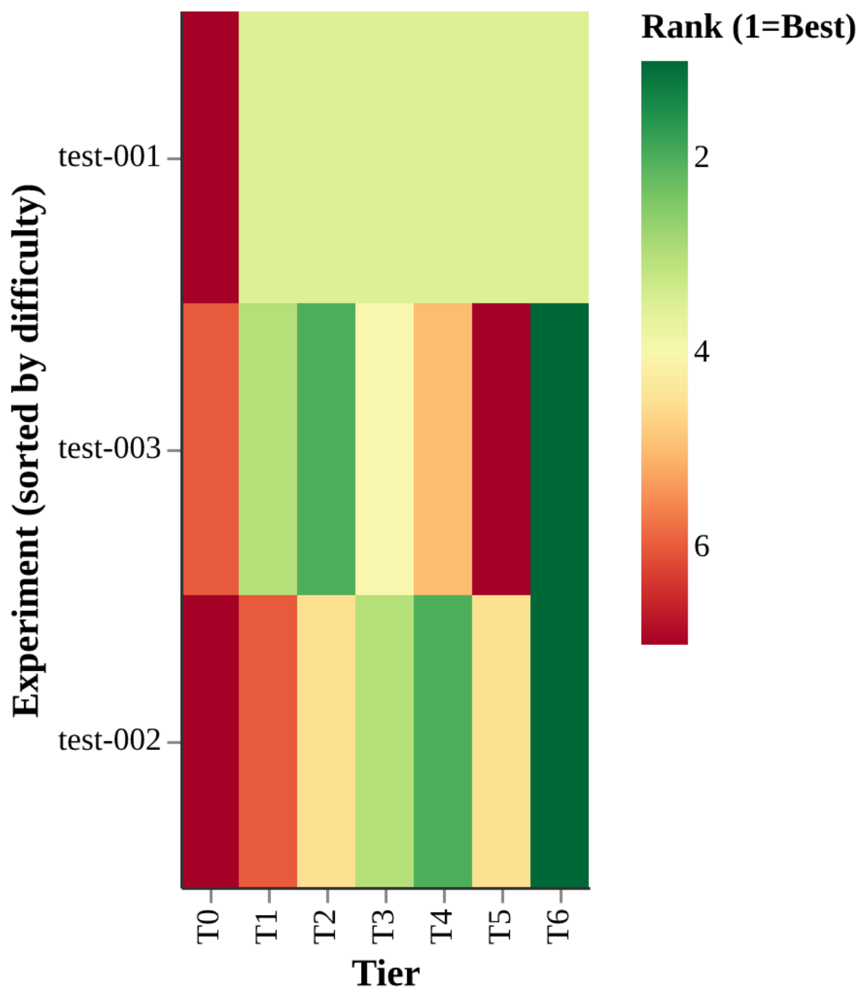
Figure 6: Tier rank stability heatmap. Each cell shows the rank of a tier (x-axis) within a given experiment (y-axis, sorted by difficulty), where rank 1 is best. Color encodes rank (green = best, red = worst). The changing color pattern across experiments indicates that tier rankings are not stable—the optimal tier varies by task, consistent with the significant tier \times experiment interaction on score.
