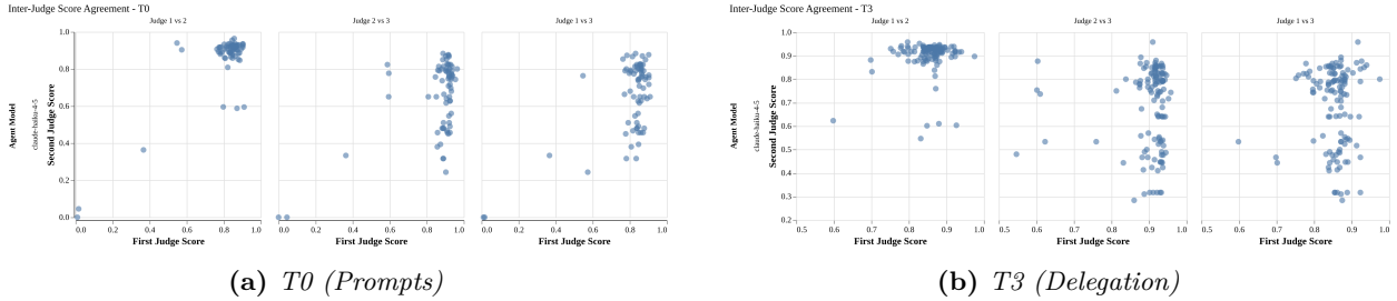
Figure 8: Judge agreement scatter plots for T0 and T3. Each point represents a run, with axes showing scores from different judge pairs. The wide scatter and lack of diagonal clustering illustrate the low inter-rater reliability across both simple (T0) and delegation-based (T3) tiers.
