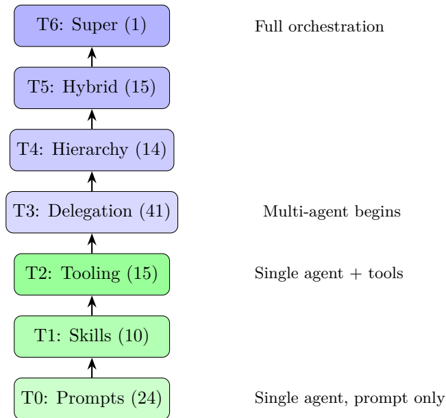
Figure 1: Scylla tier hierarchy. Green tiers (T0–T2) represent single-agent configurations; blue tiers (T3–T6) introduce multi-agent coordination. All tiers achieve comparable pass rates (0.935–1.000) in this study.
