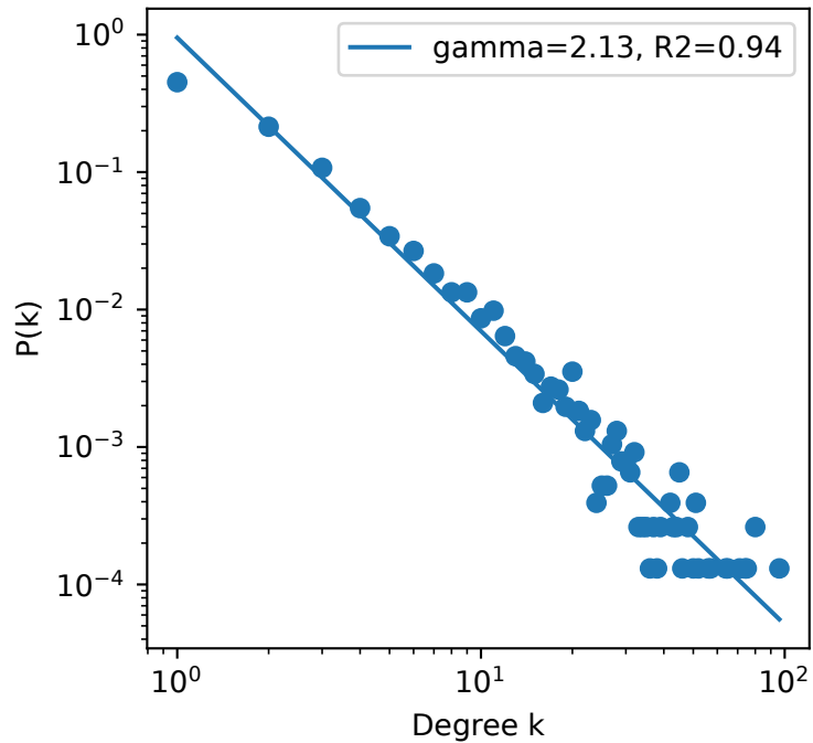
in-degree distribution
