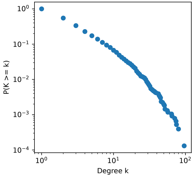
in-degree CCDF
