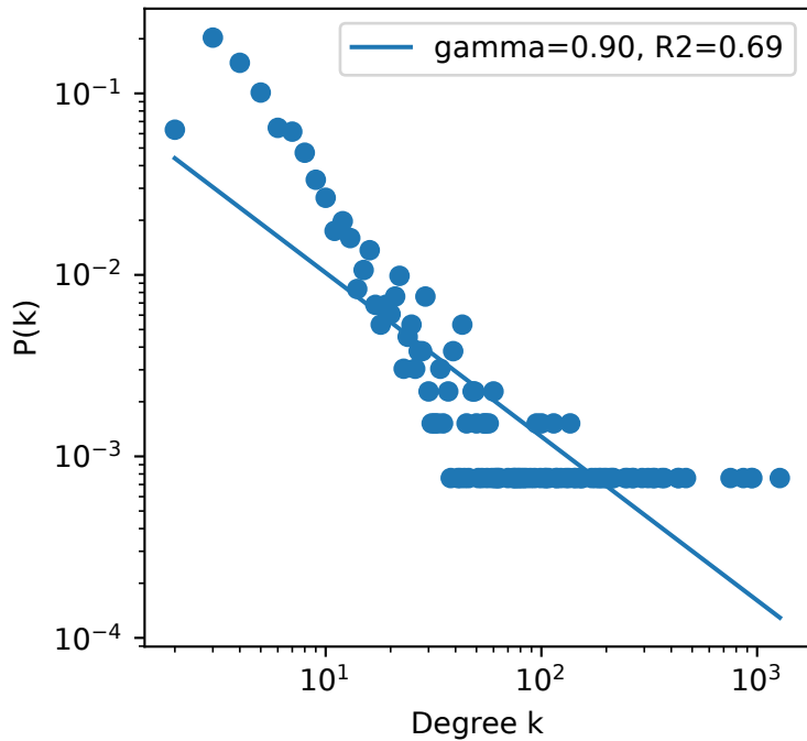
out-degree distribution
