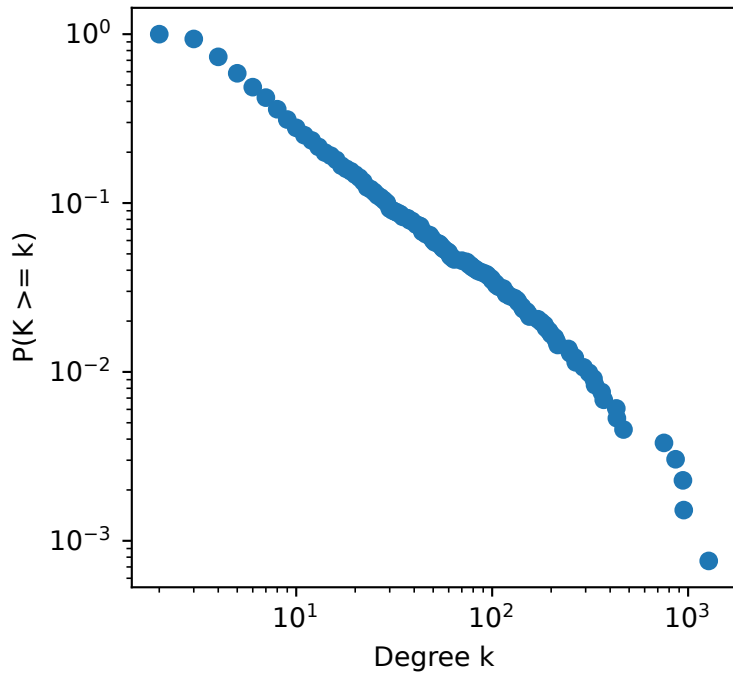
out-degree CCDF
