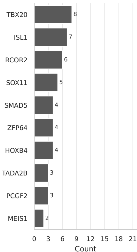
Upstream nodes
