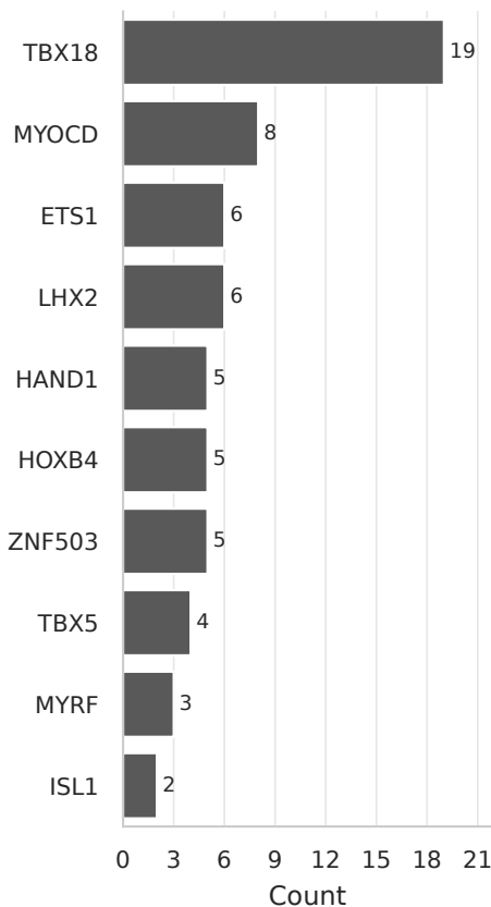
Downstream nodes
