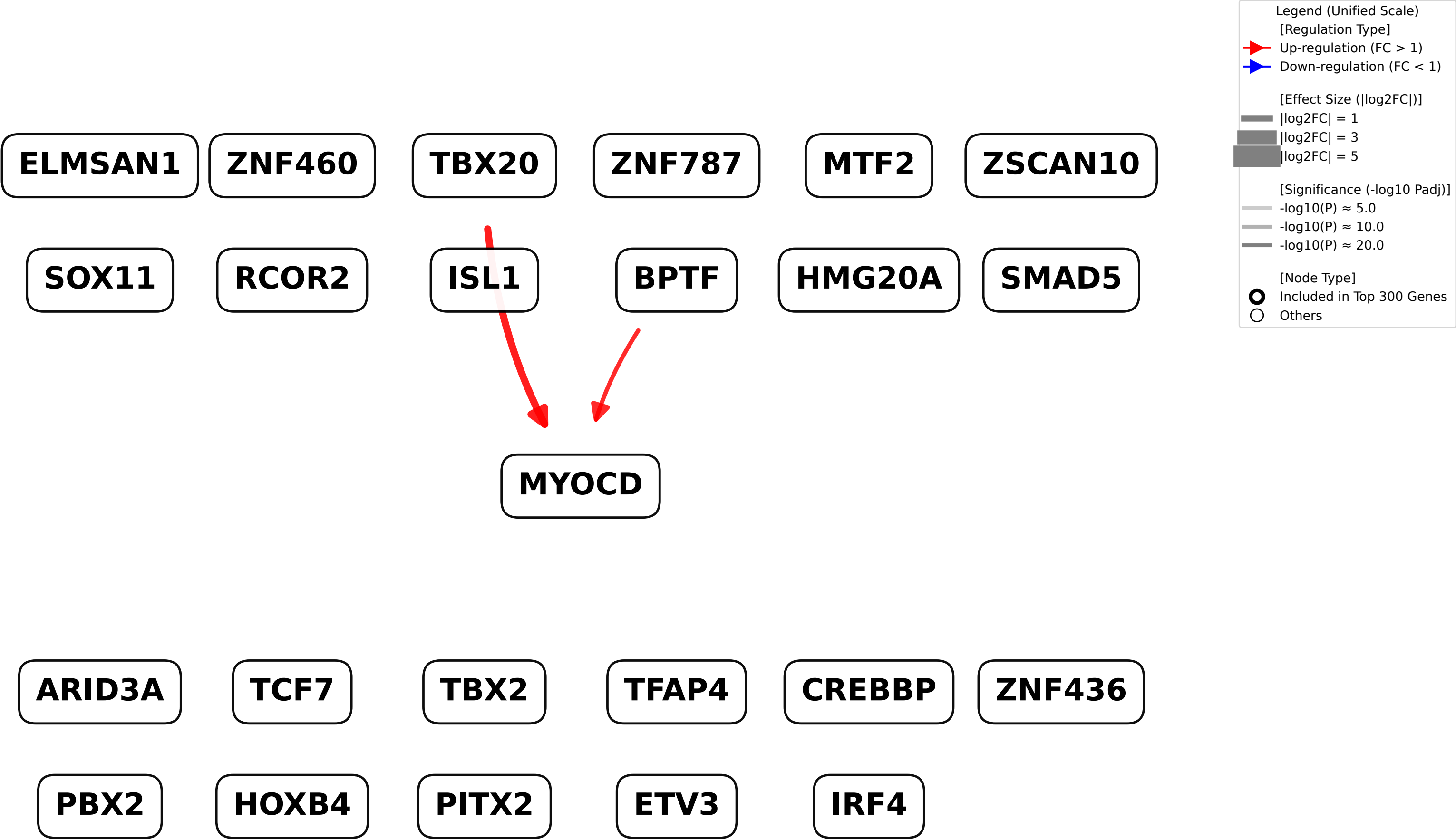
TF-TF Regulatory Network around D29:Usage1
