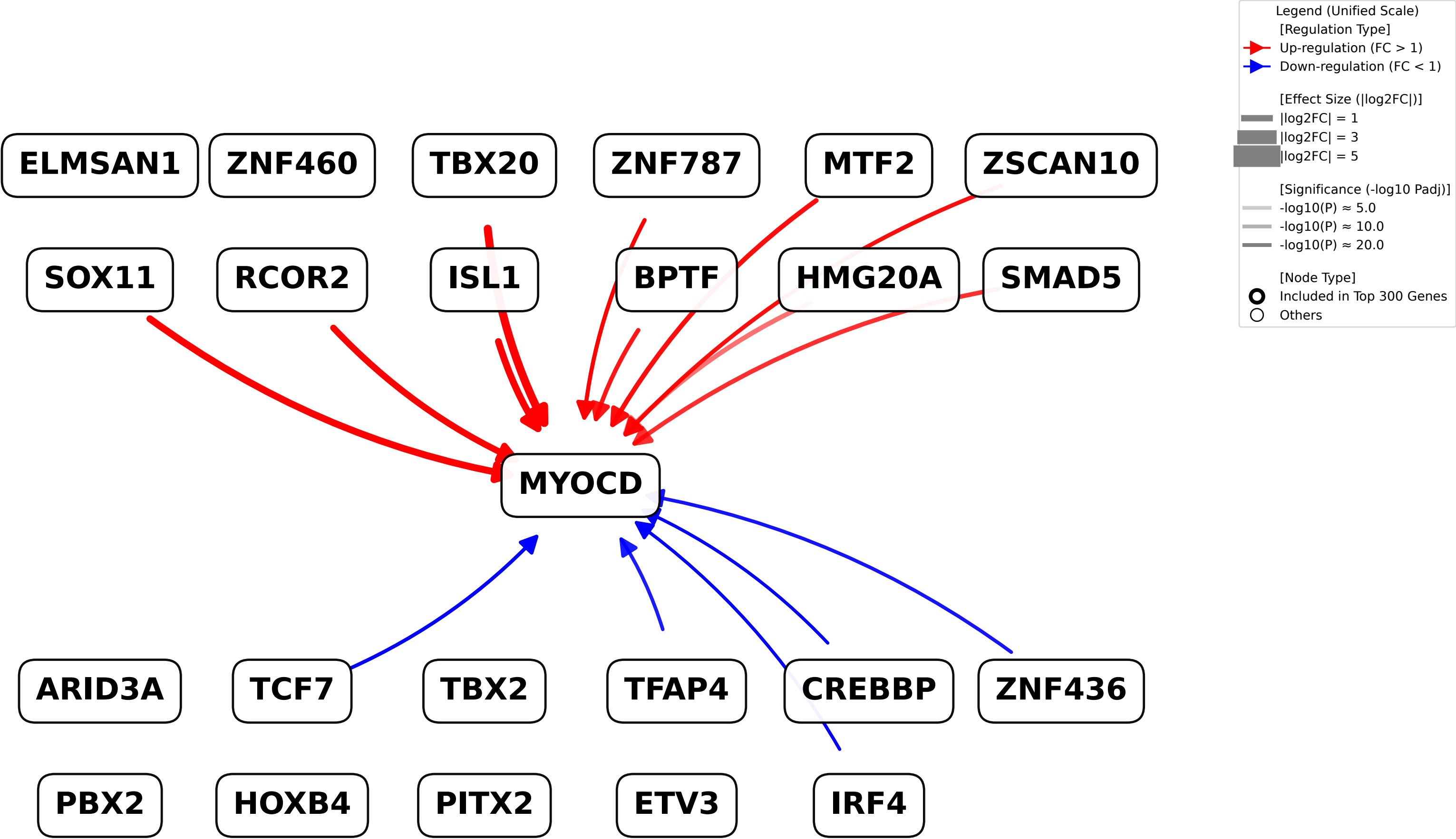
TF-TF Regulatory Network around D12:Usage1
