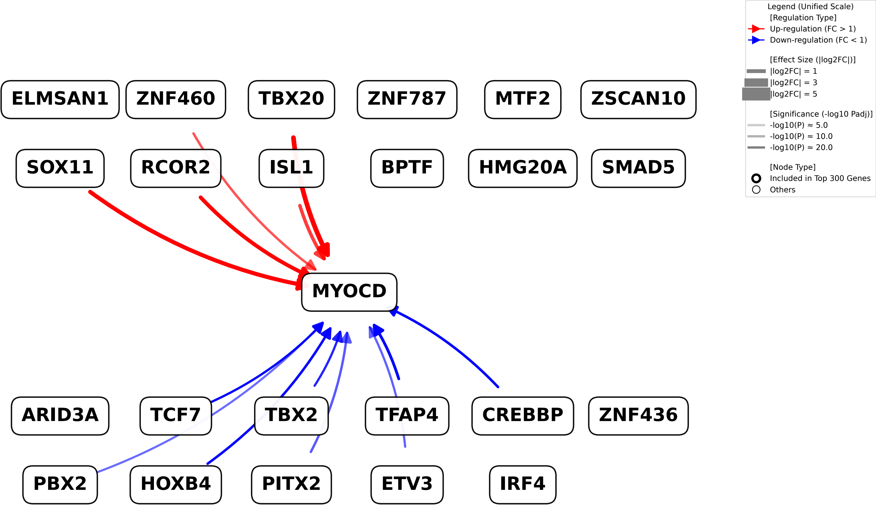
TF-TF Regulatory Network around D8:Usage1
