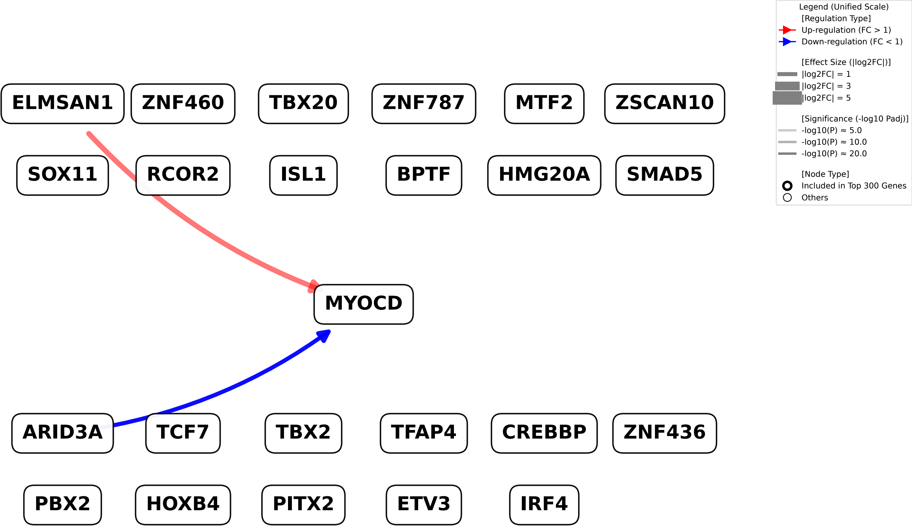
TF-TF Regulatory Network around D4:Usage1
