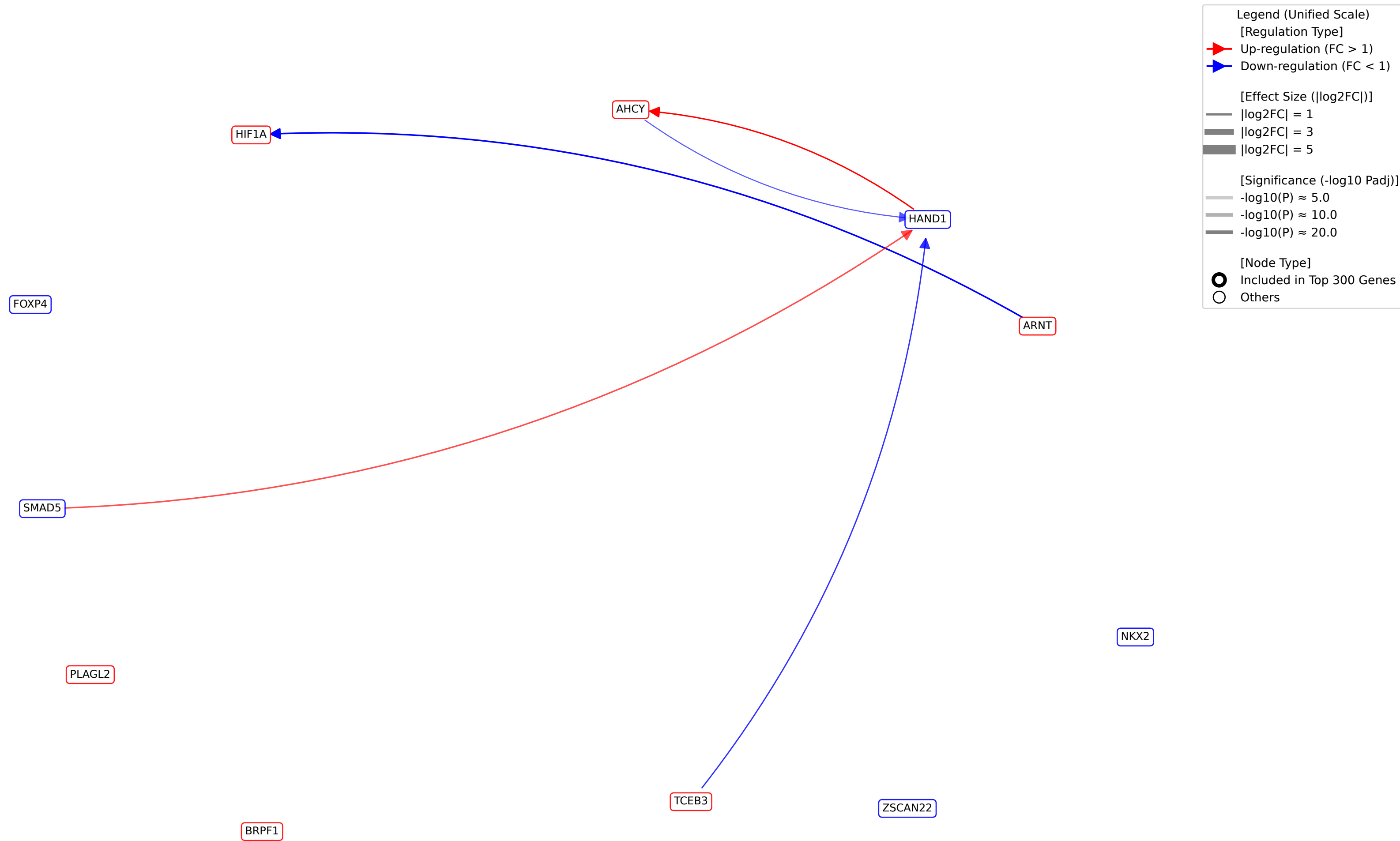
TF-TF Regulatory Network around Usage_192_total
