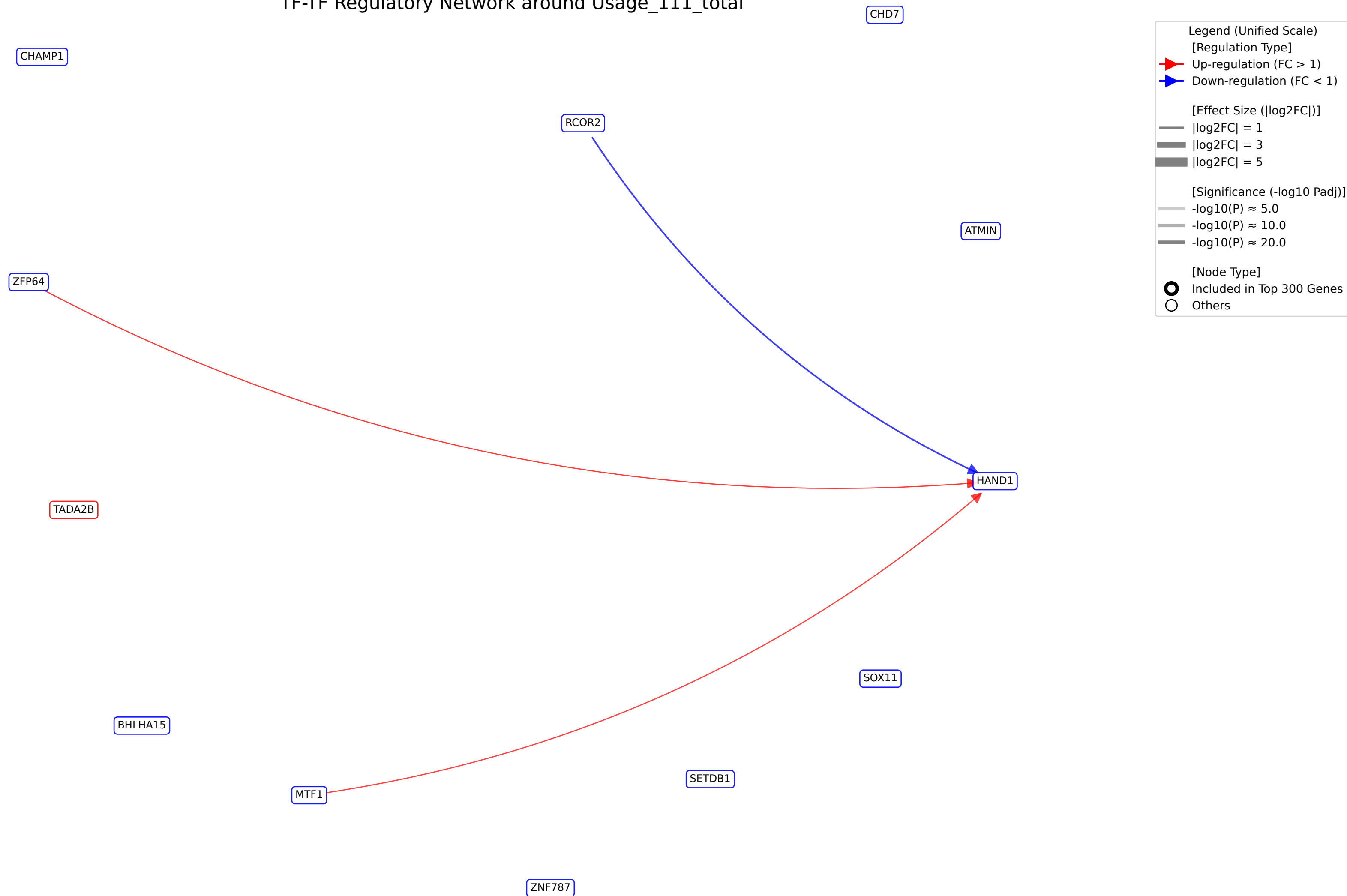
TF-TF Regulatory Network around Usage_111_total
