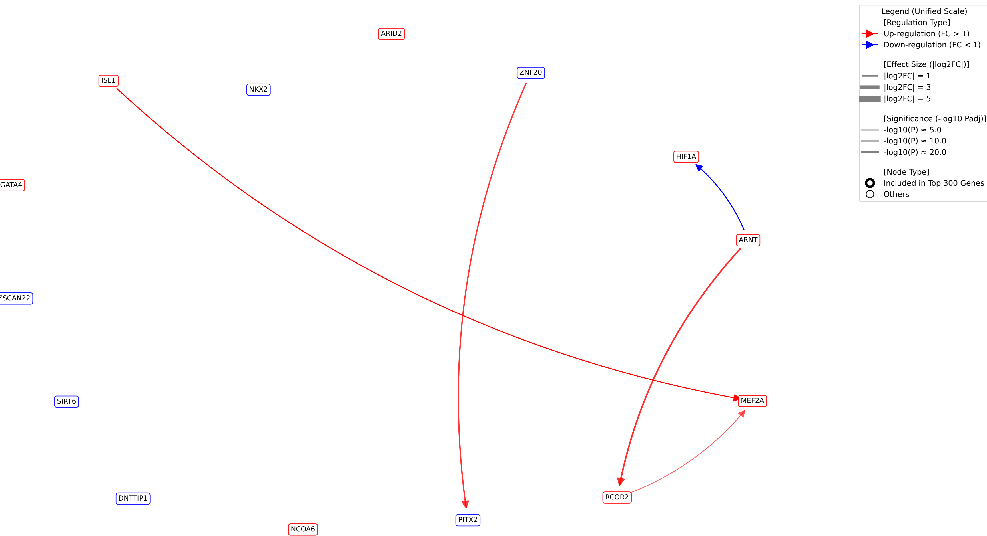
TF-TF Regulatory Network around Usage_50_total
