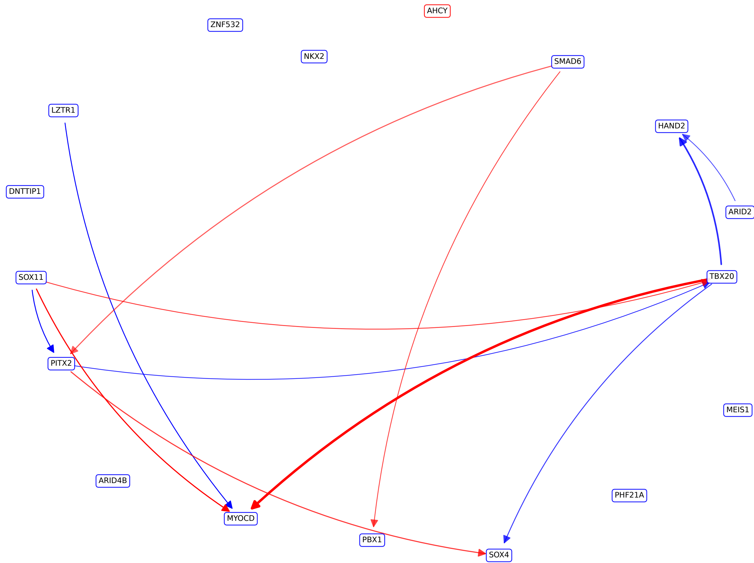
TF-TF Regulatory Network around Usage_33_total
