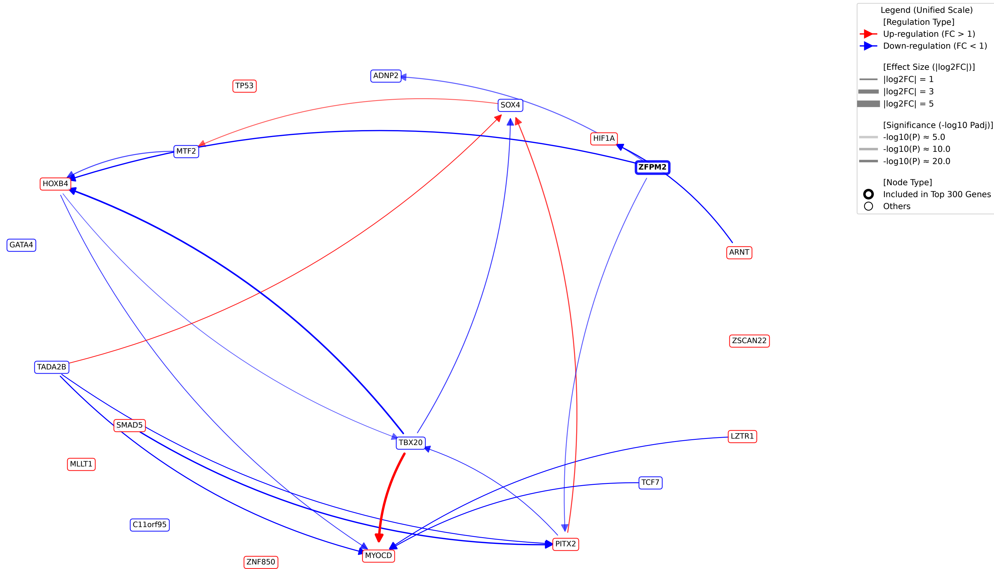
TF-TF Regulatory Network around Usage_36_total
