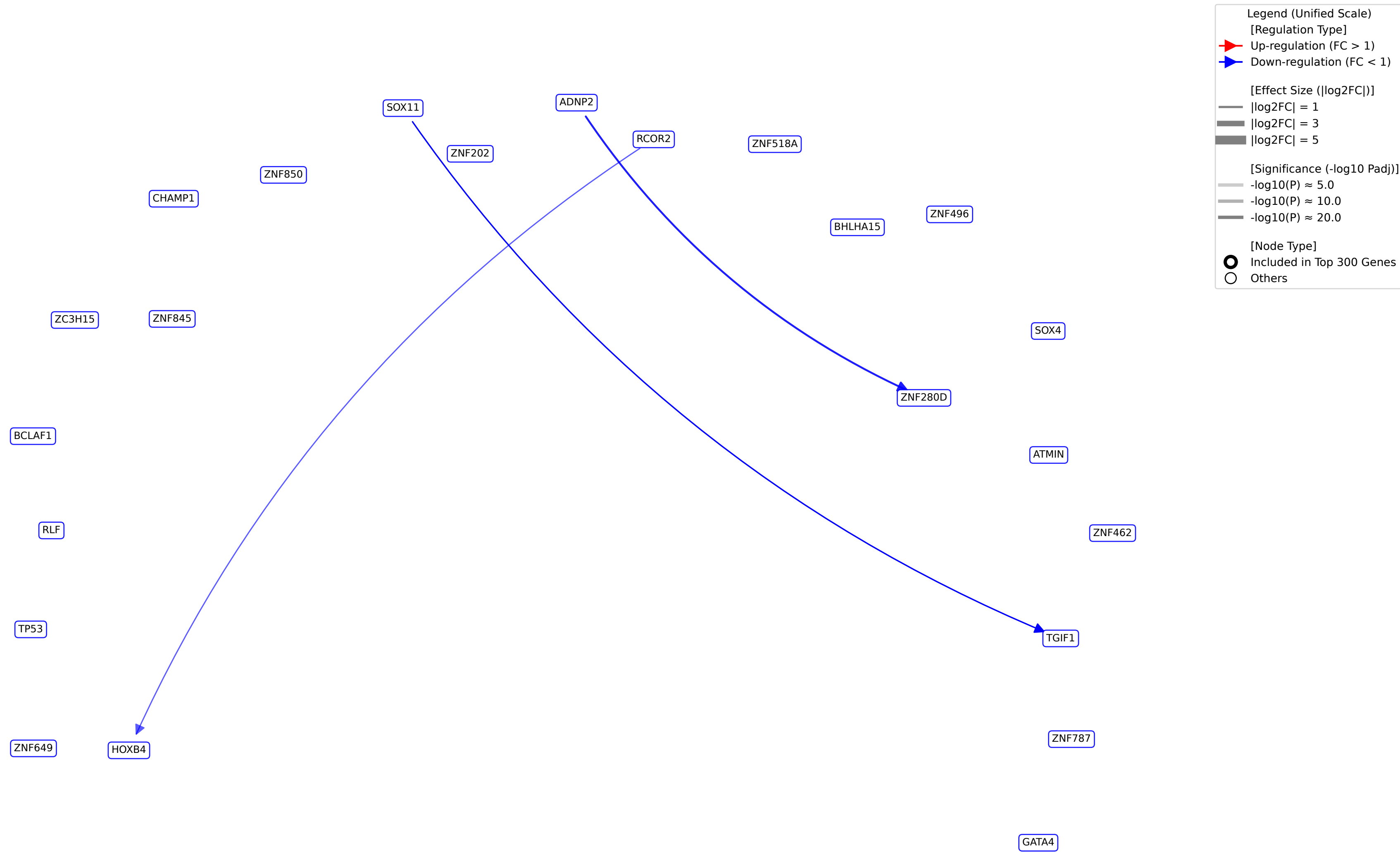
TF-TF Regulatory Network around Usage_39_total
