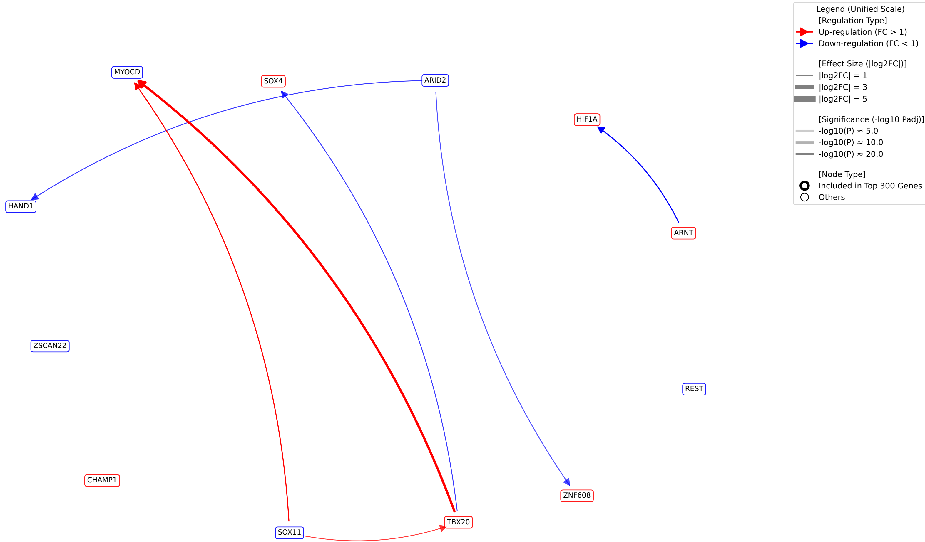
TF-TF Regulatory Network around Usage_67_total
