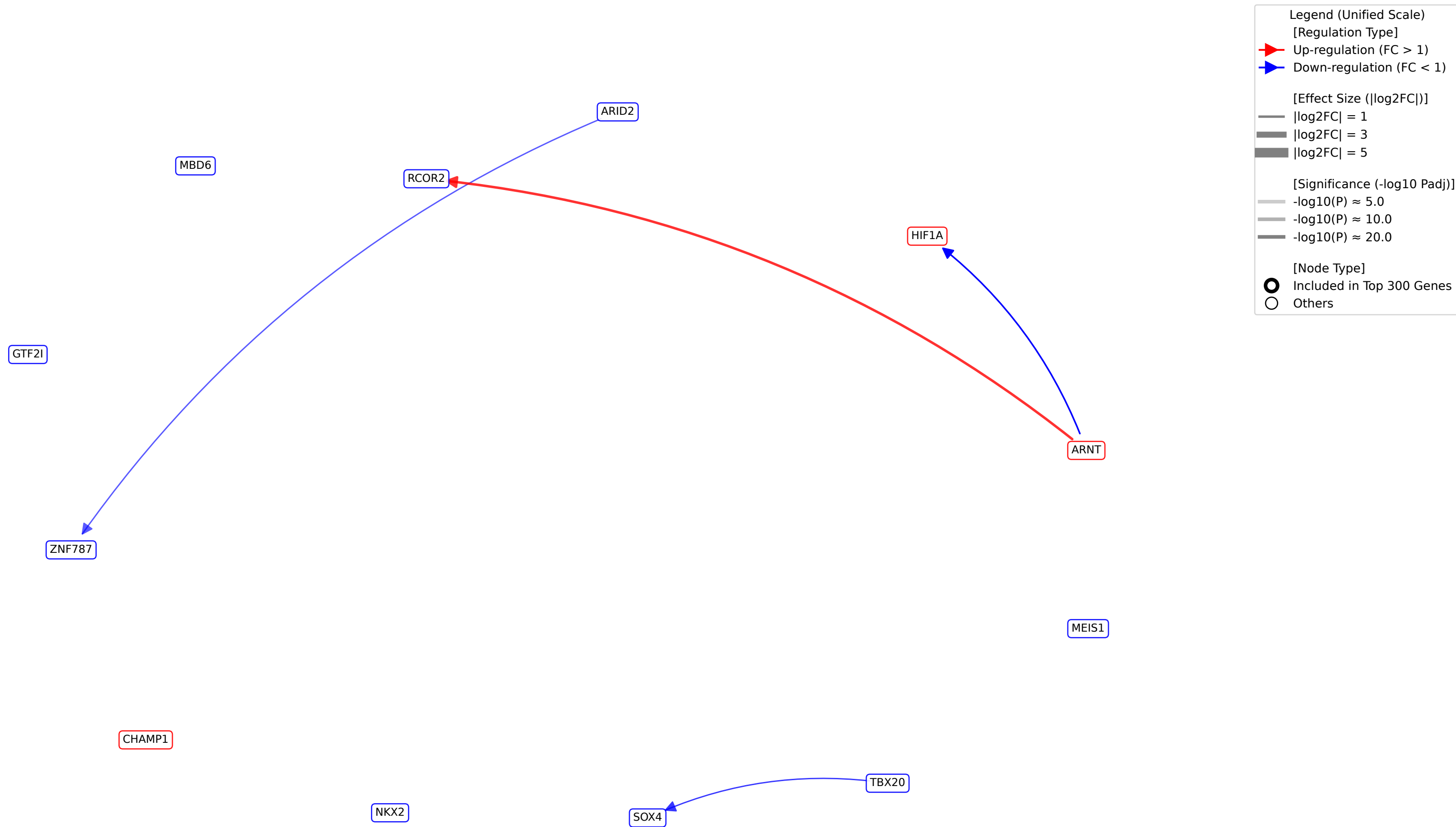
TF-TF Regulatory Network around Usage_22_total
