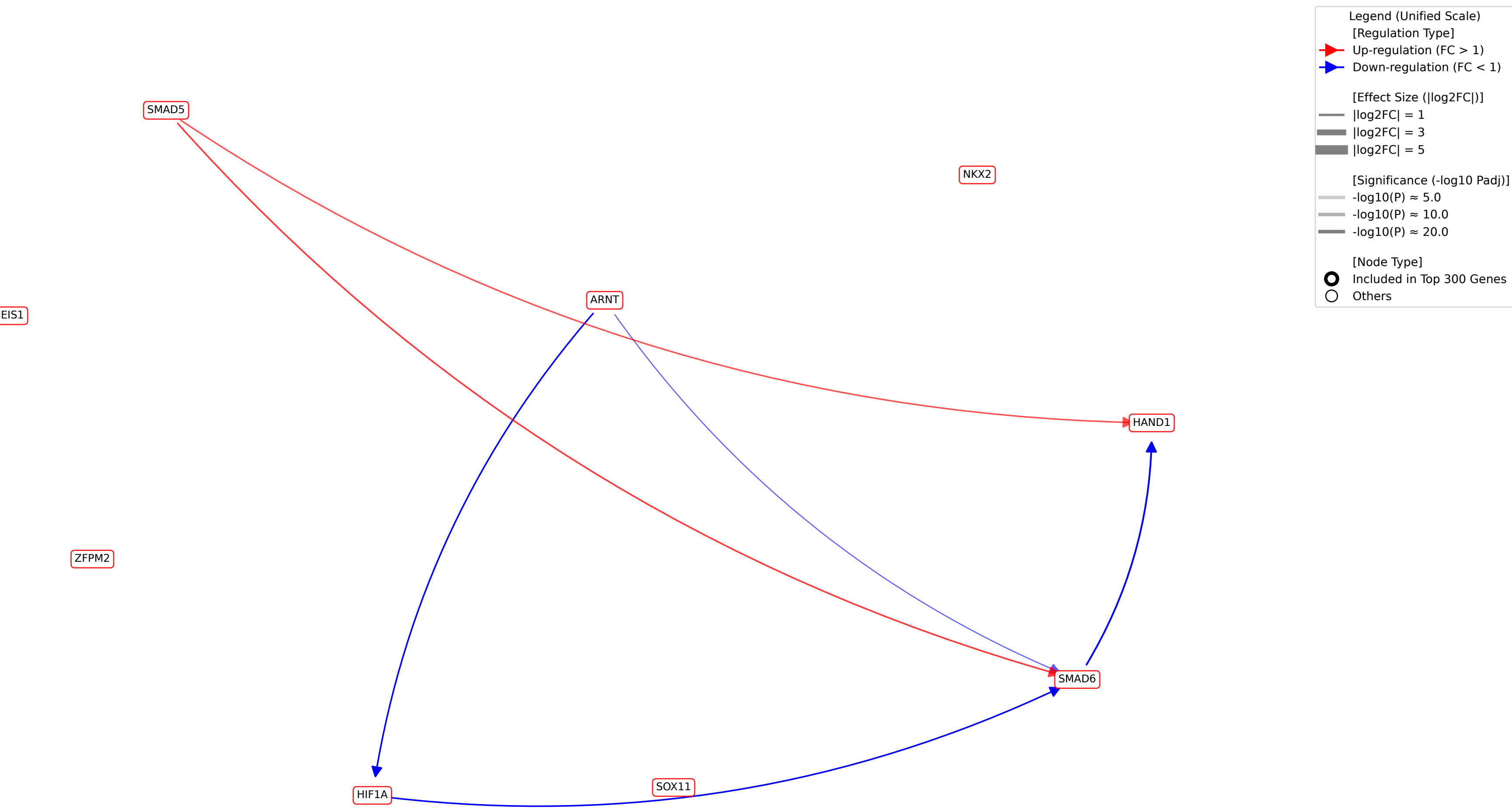
TF-TF Regulatory Network around Usage_145_total
