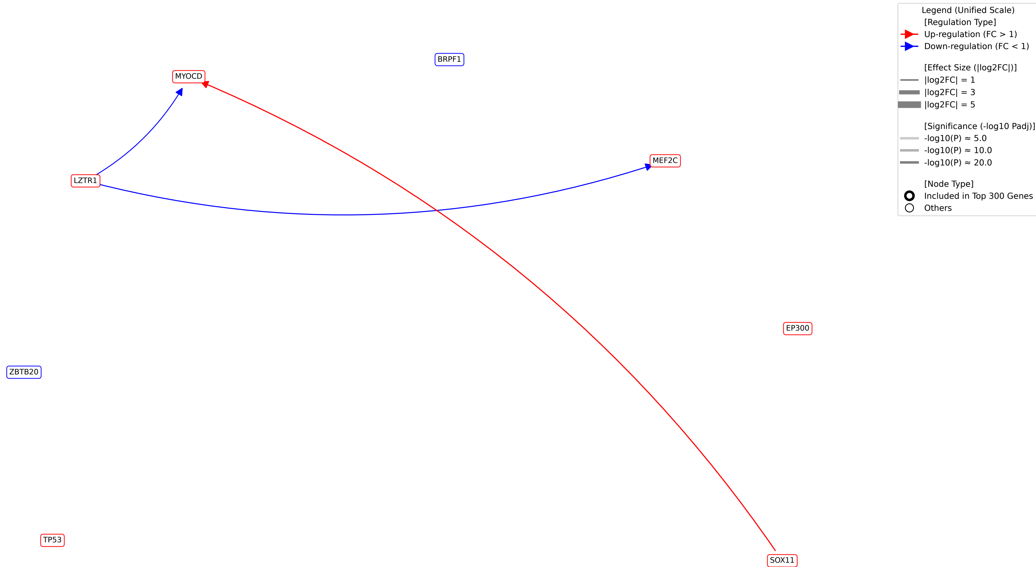
TF-TF Regulatory Network around Usage_189_total
