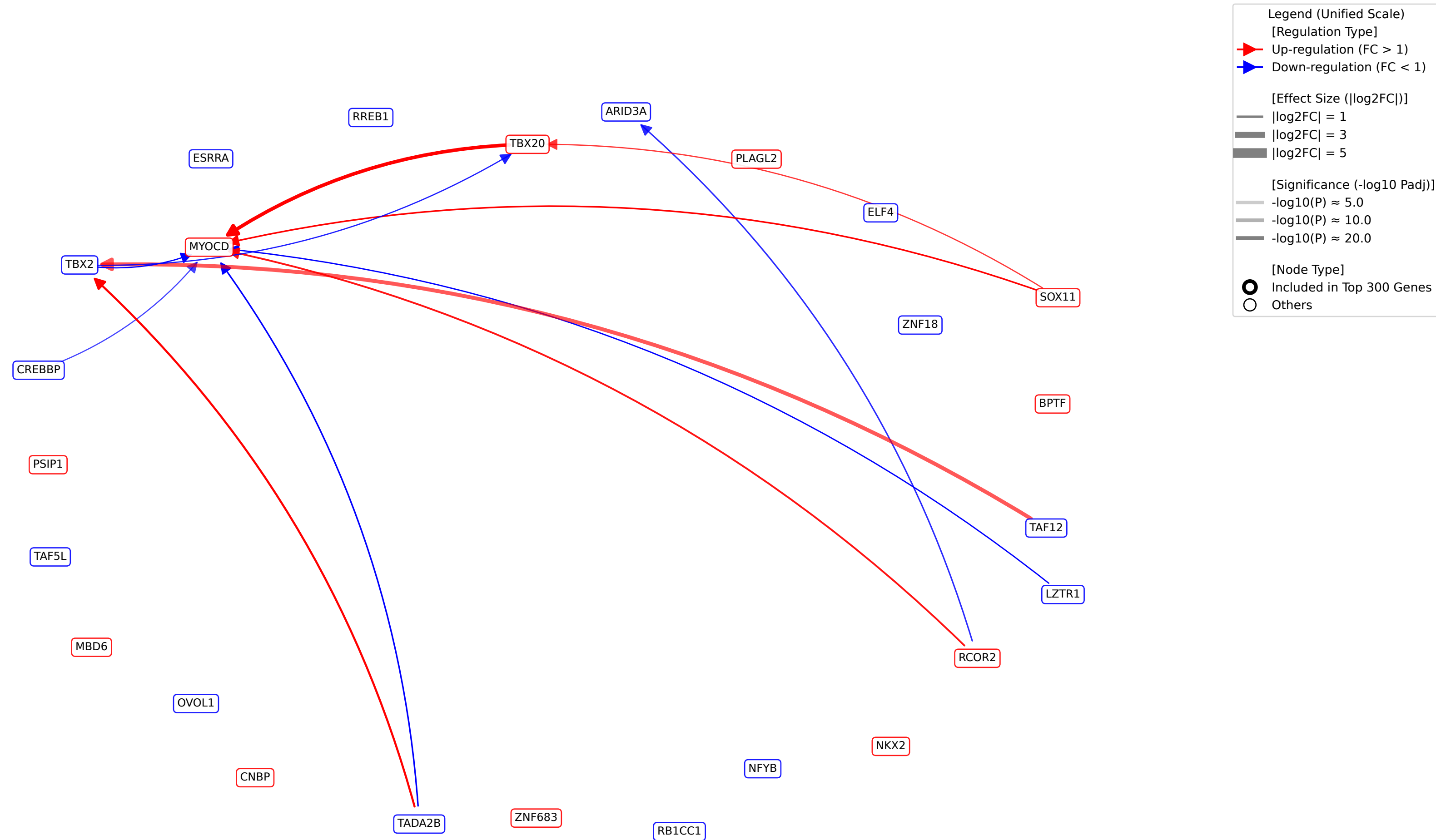
TF-TF Regulatory Network around Usage_11_total
