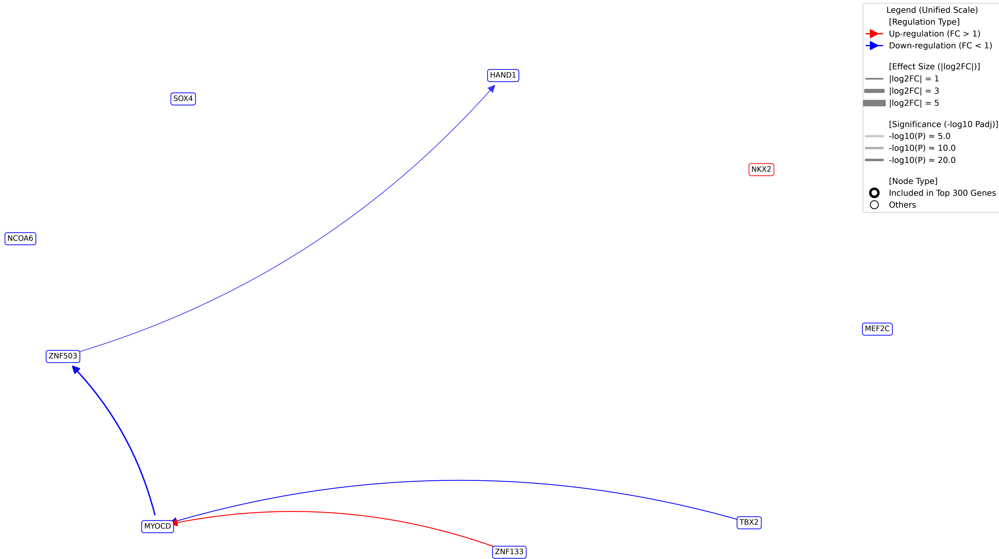
TF-TF Regulatory Network around Usage_120_total
