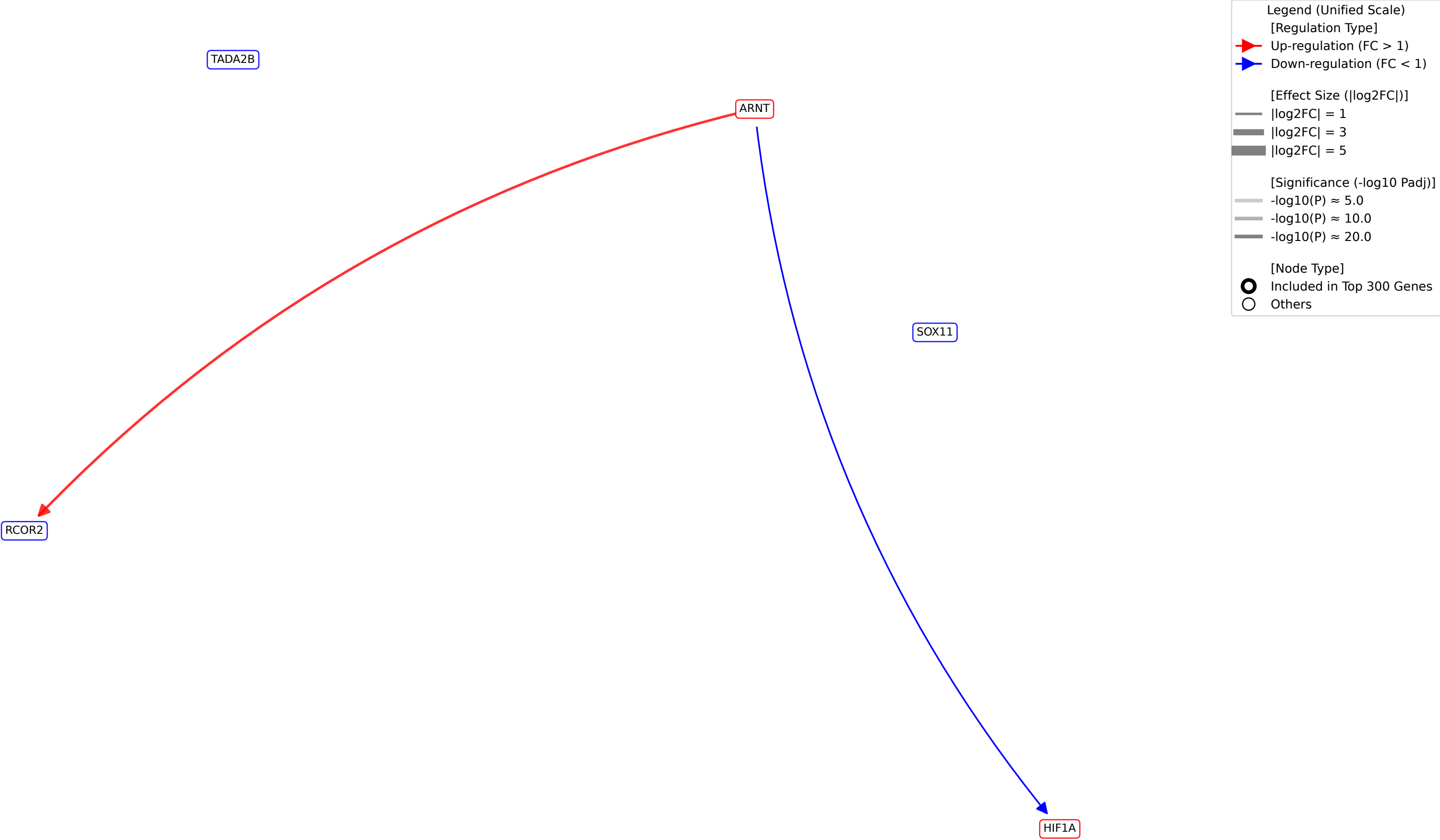
TF-TF Regulatory Network around Usage_123_total
