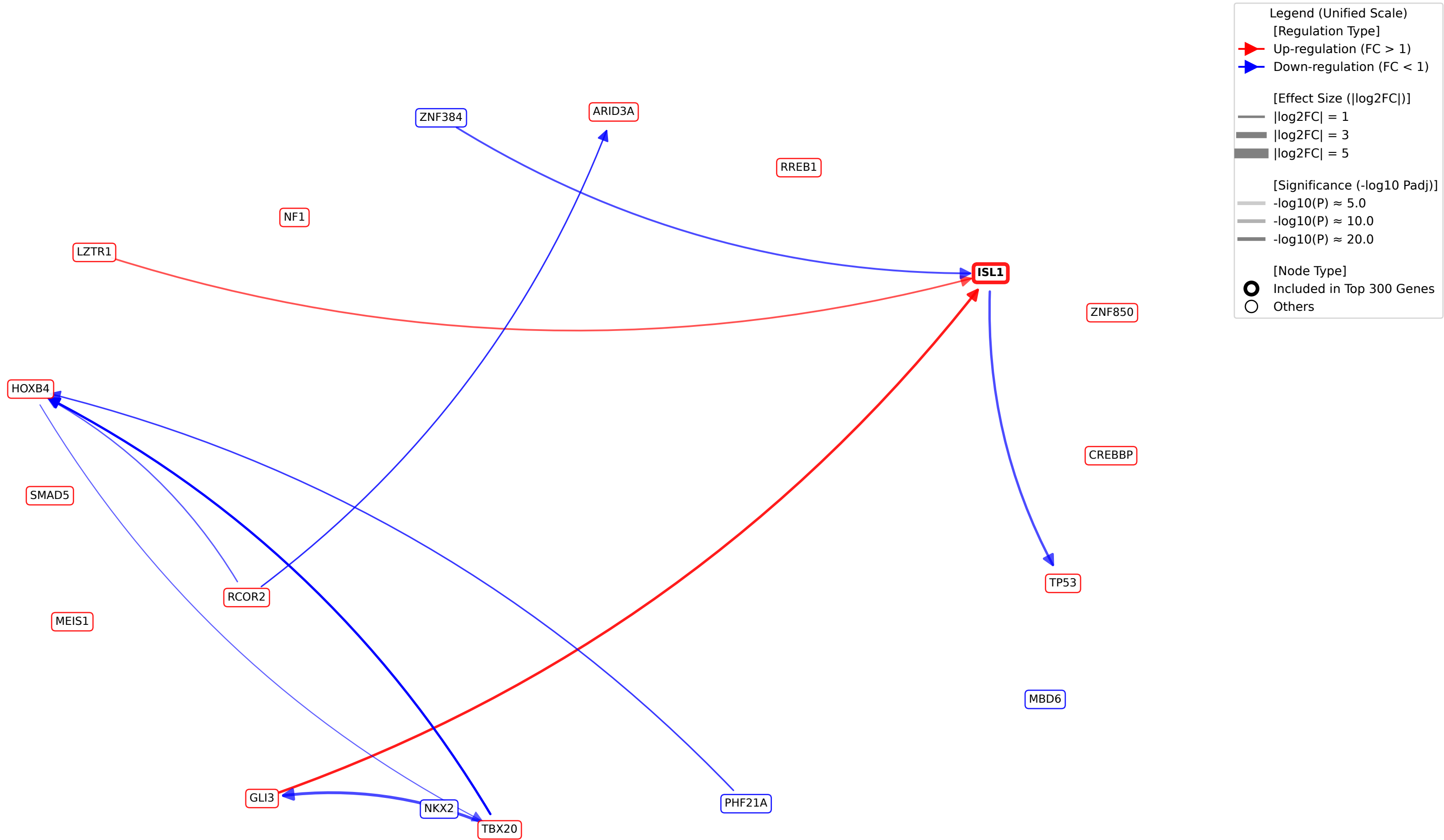
TF-TF Regulatory Network around Usage_6_total
