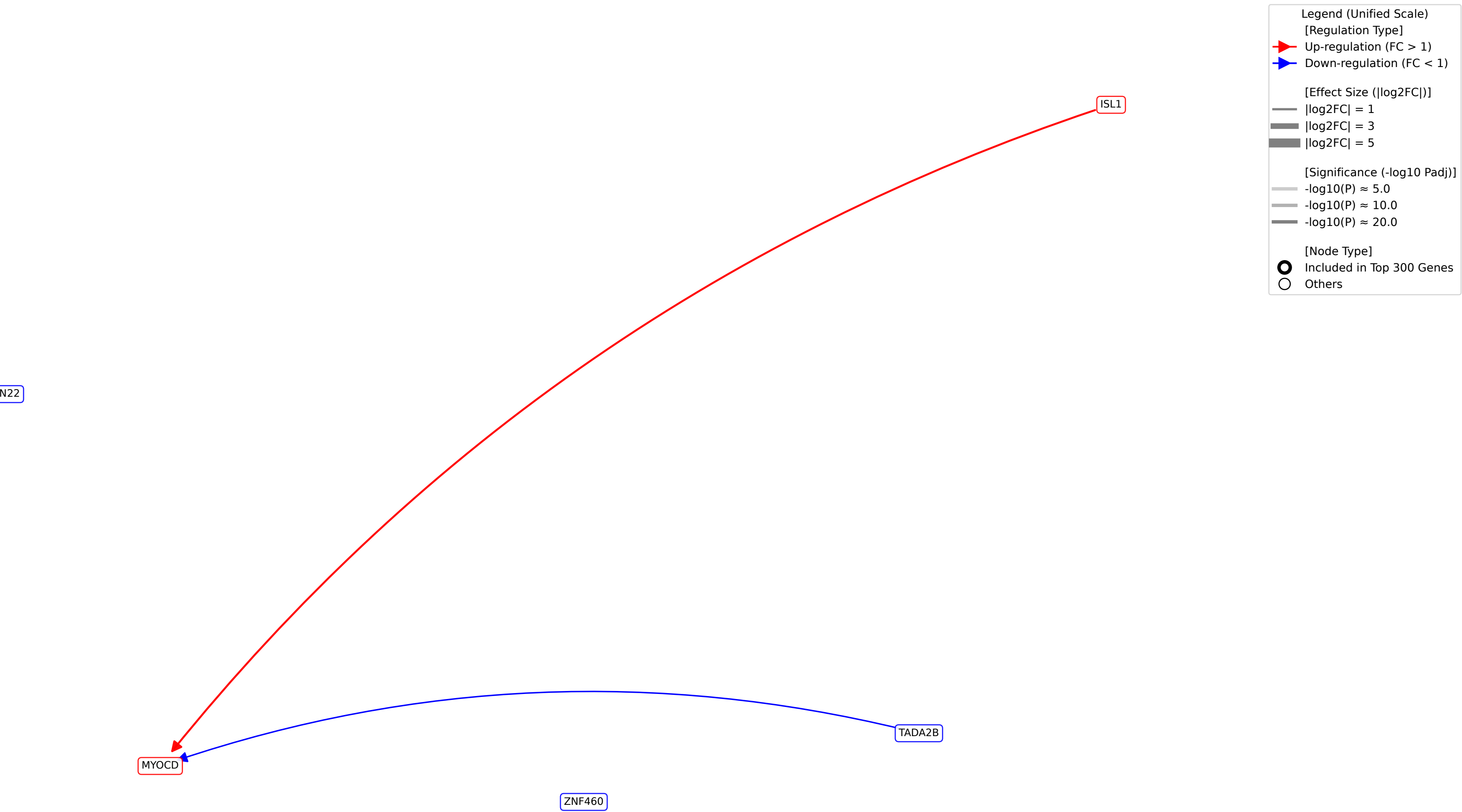
TF-TF Regulatory Network around Usage_47_total
