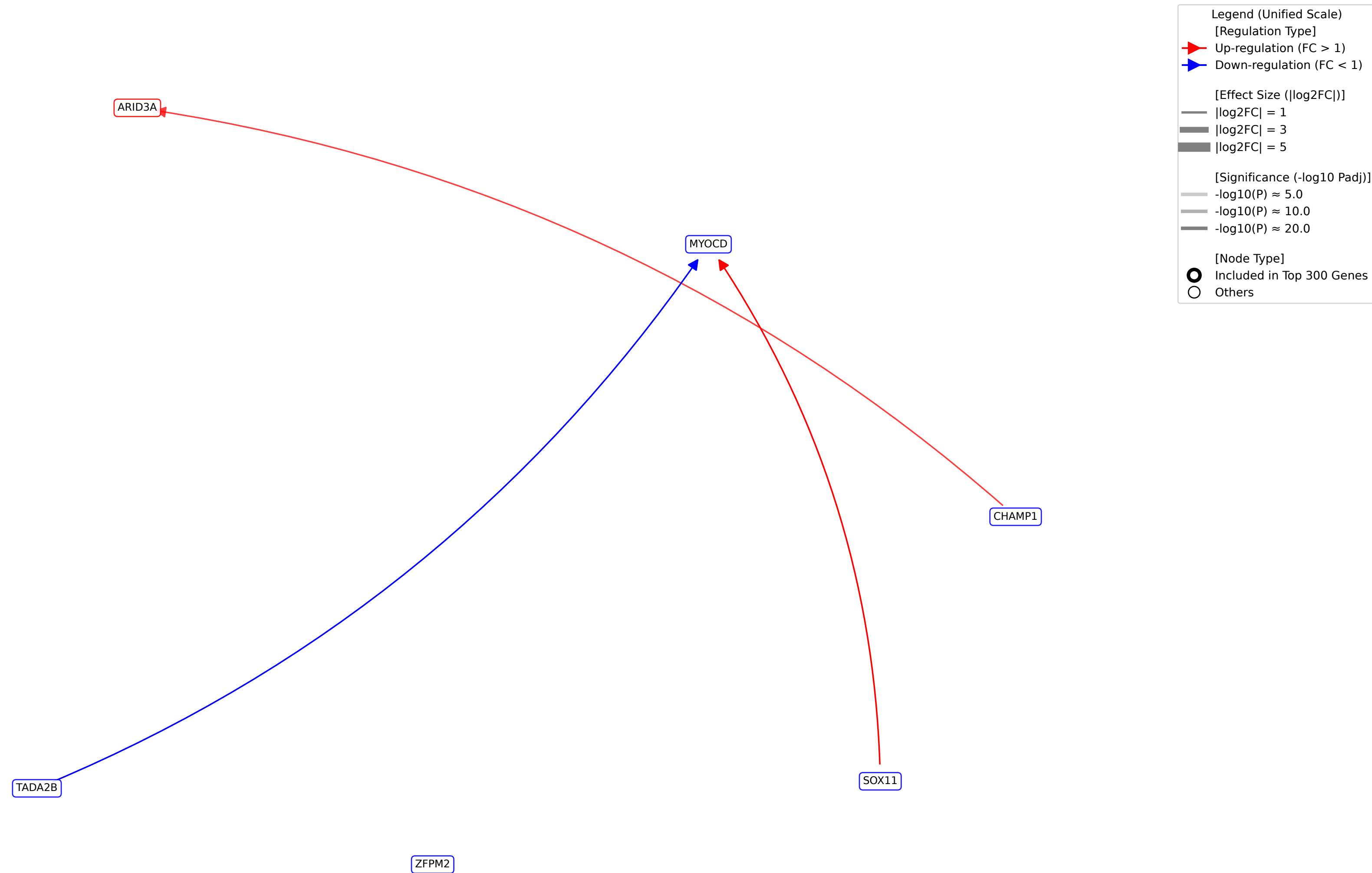
TF-TF Regulatory Network around Usage_18_total
