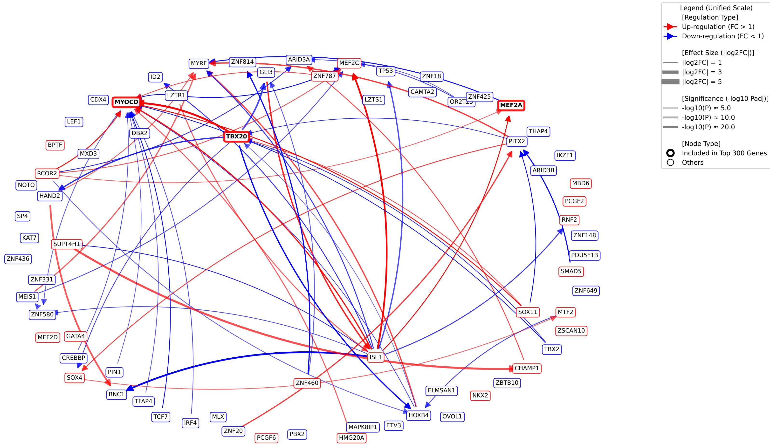
TF-TF Regulatory Network around Usage_1_total
