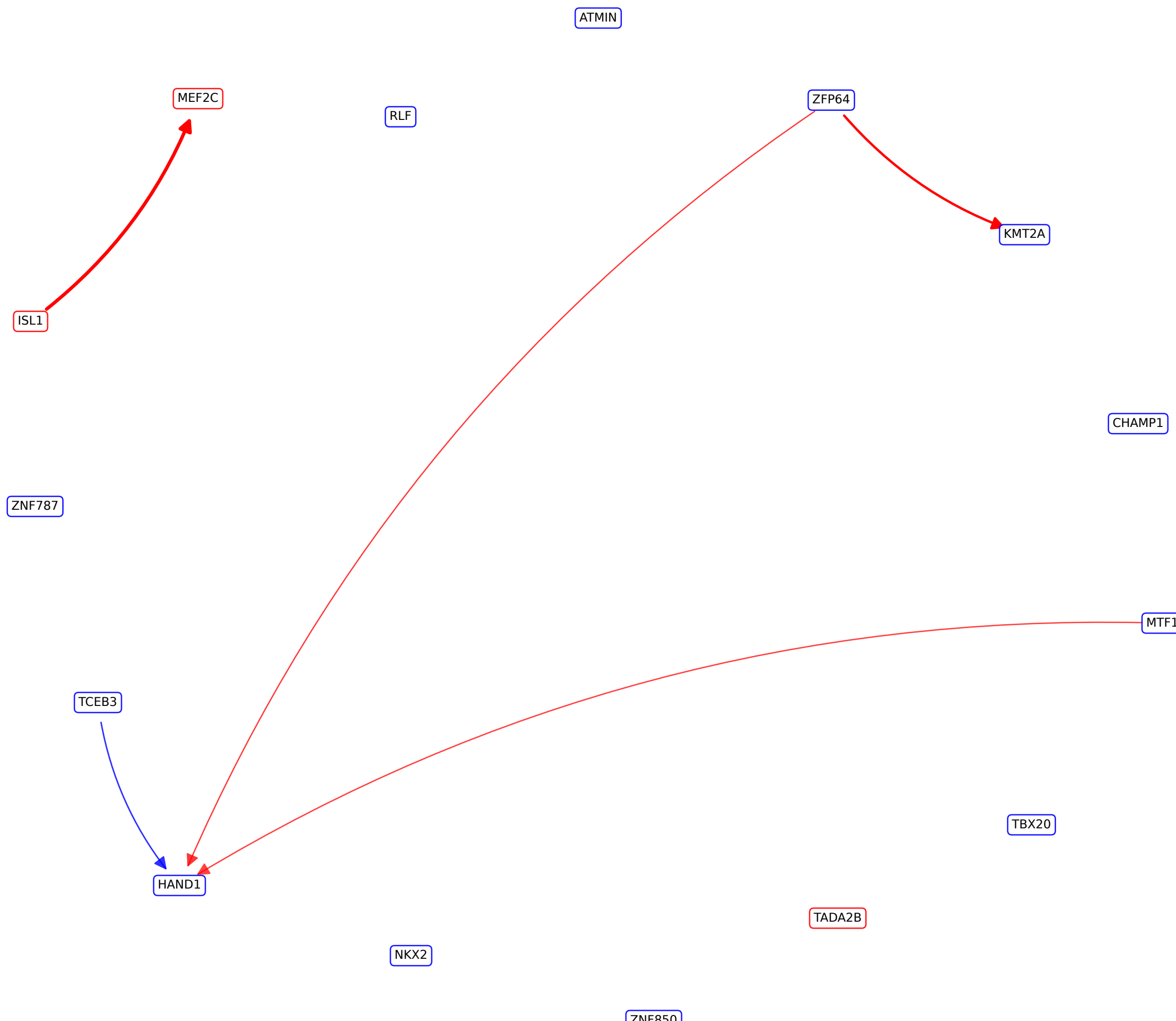
TF-TF Regulatory Network around Usage_235_total
