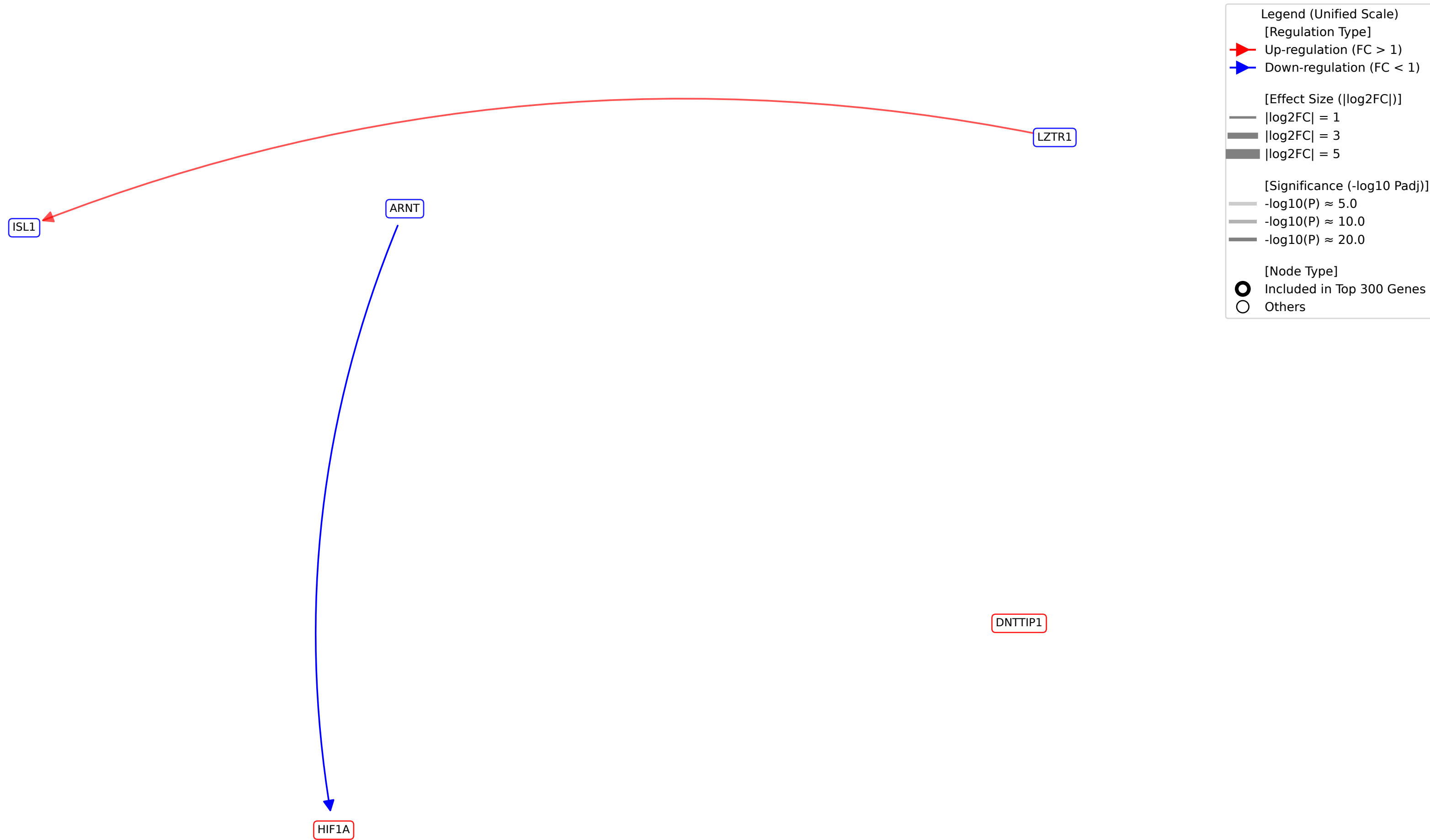
TF-TF Regulatory Network around Usage_158_total
