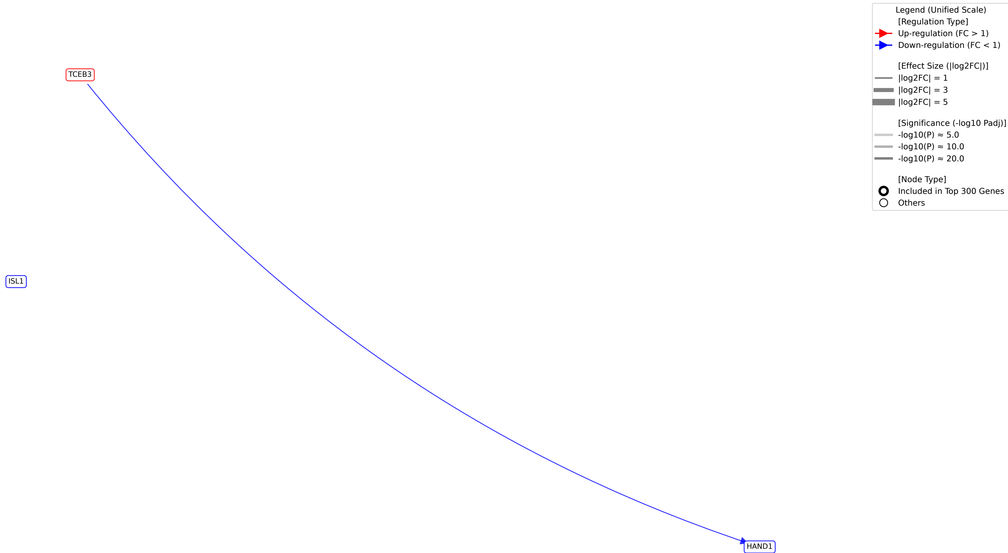
TF-TF Regulatory Network around Usage_185_total
