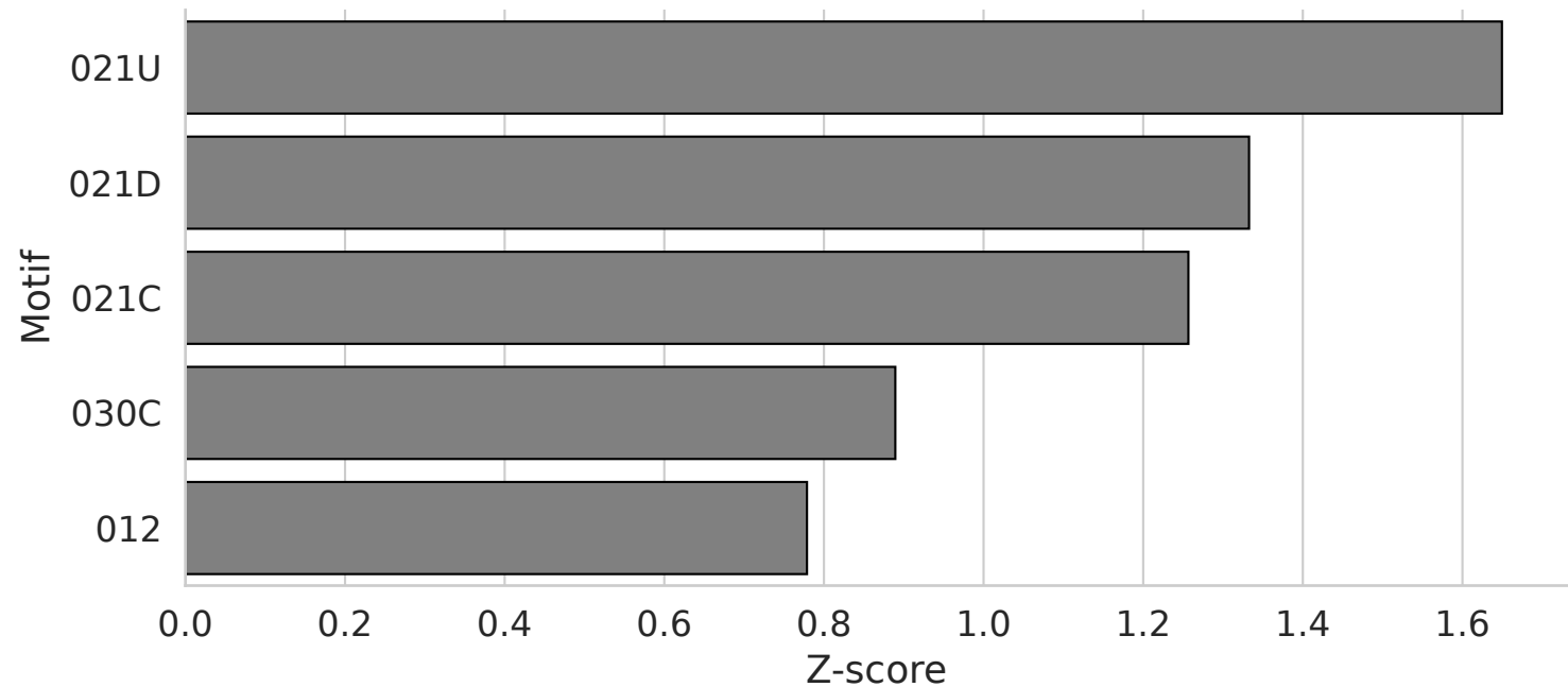
Motif Enrichment Z-scores
