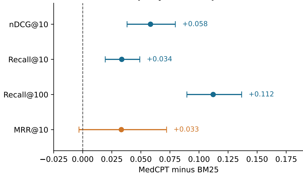
Paired query bootstrap, 95% CI
