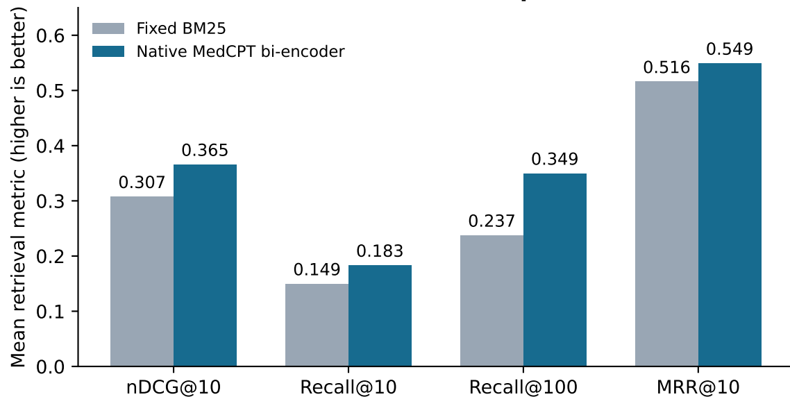
All 323 official test queries
