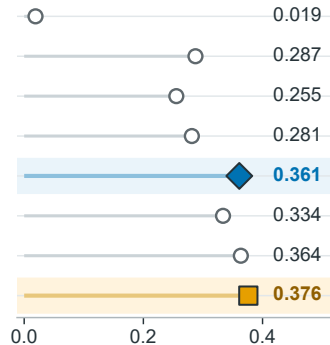
(b) Raw NDCG@10: CE wins
