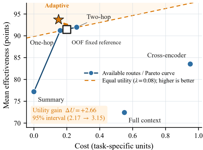
D. 2Wiki-Structured
