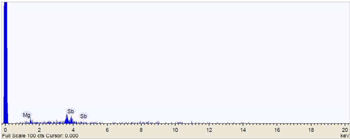
Antimony positive electrode
