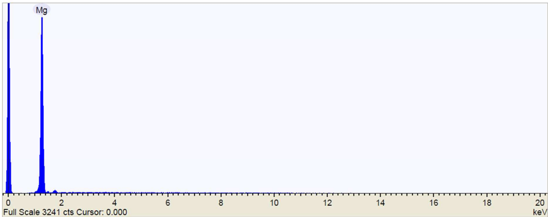
Magnesium negative electrode
