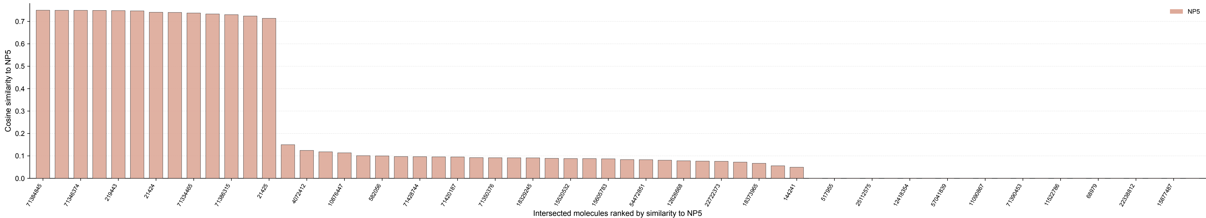
Similarity of intersected molecules to NP5 (N = 62)
