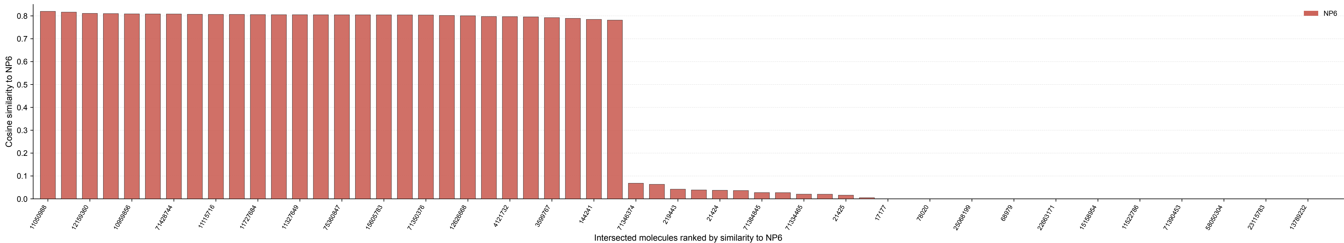
Similarity of intersected molecules to NP6 (N = 62)
