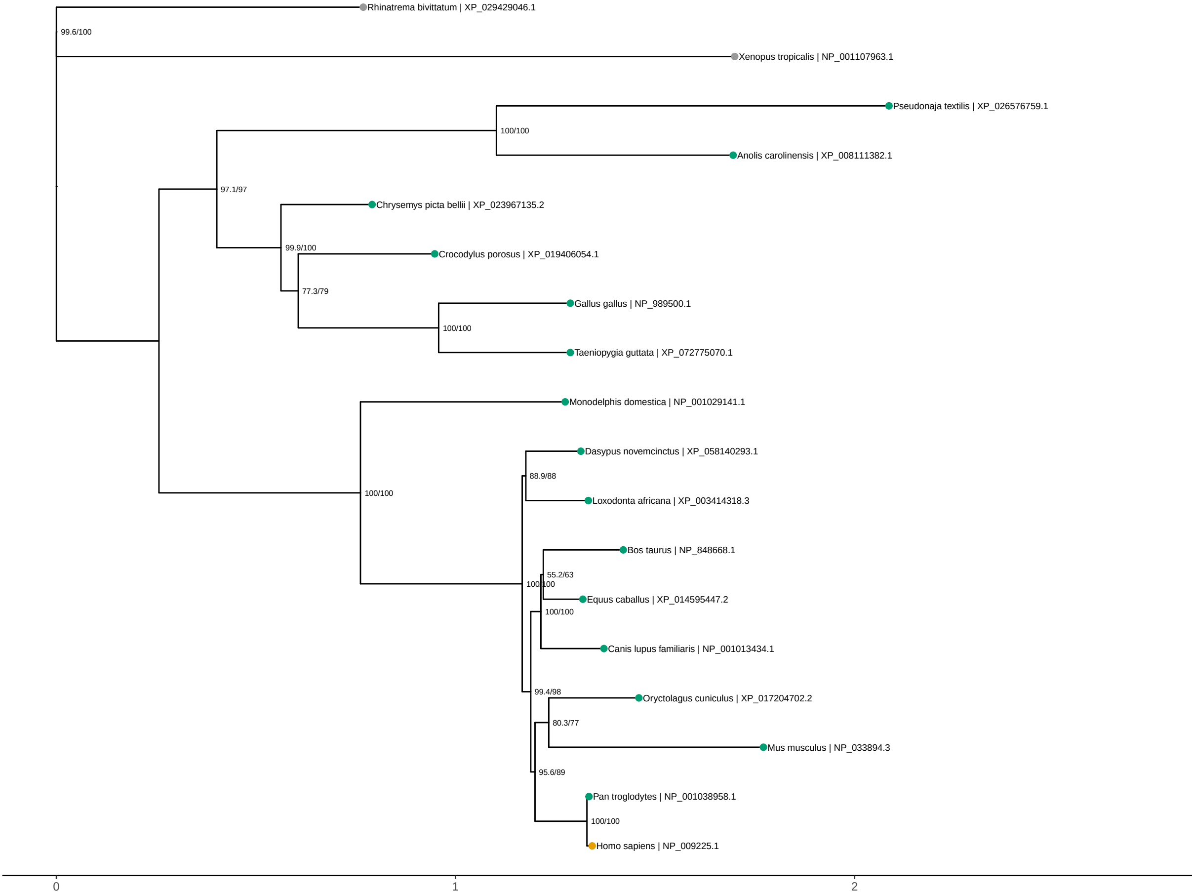
Gene tree; root state declared as outgroup-rooted. Branches: substitutions per site. Tip order was not ladderized. Support: sh-amlr/ufboot.
