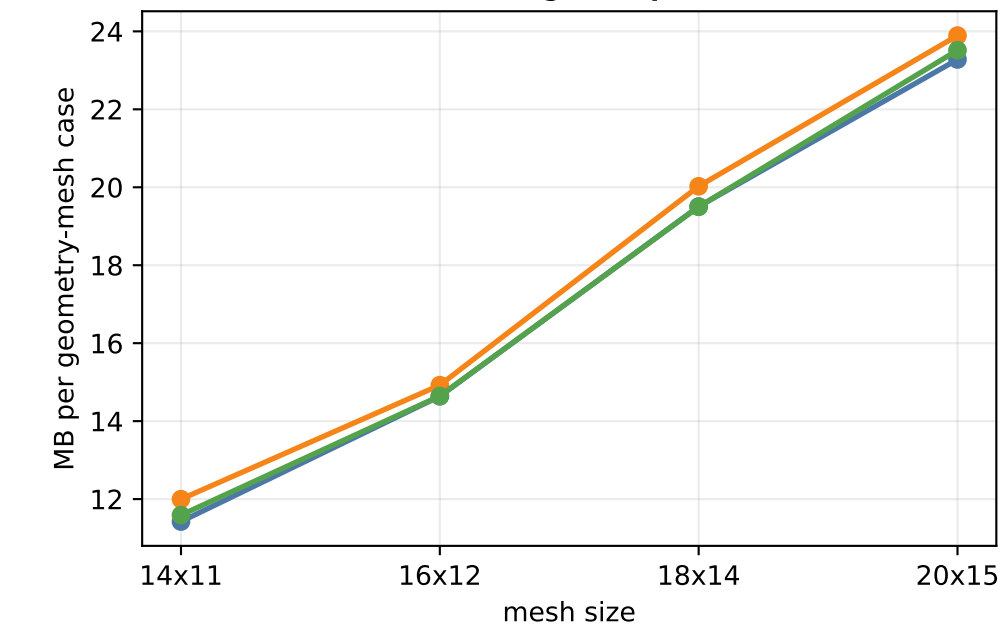
(c) storage footprint
